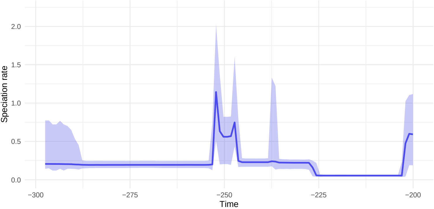
Speciation (combined_10_mcmc)
