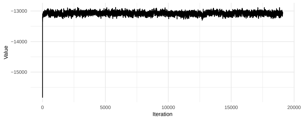
Prior Trace
