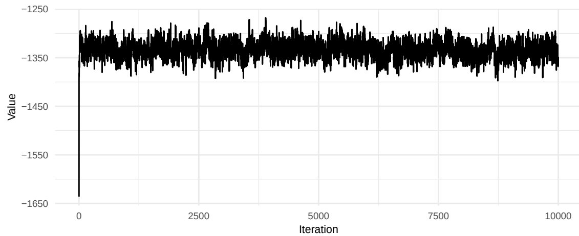
K birth Trace
