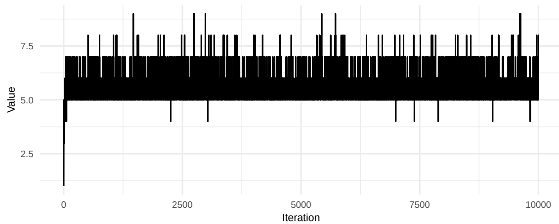
K death Trace
