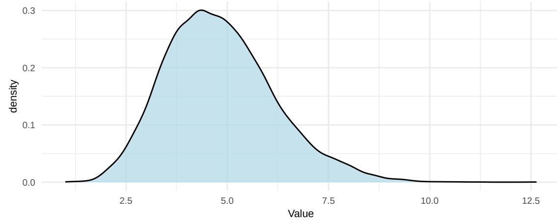
RJ hp Density
