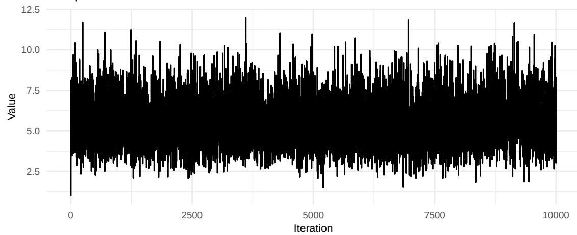
RJ hp Trace
