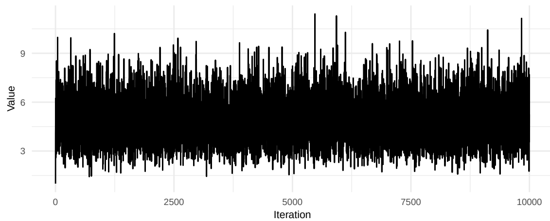
RJ hp Trace
