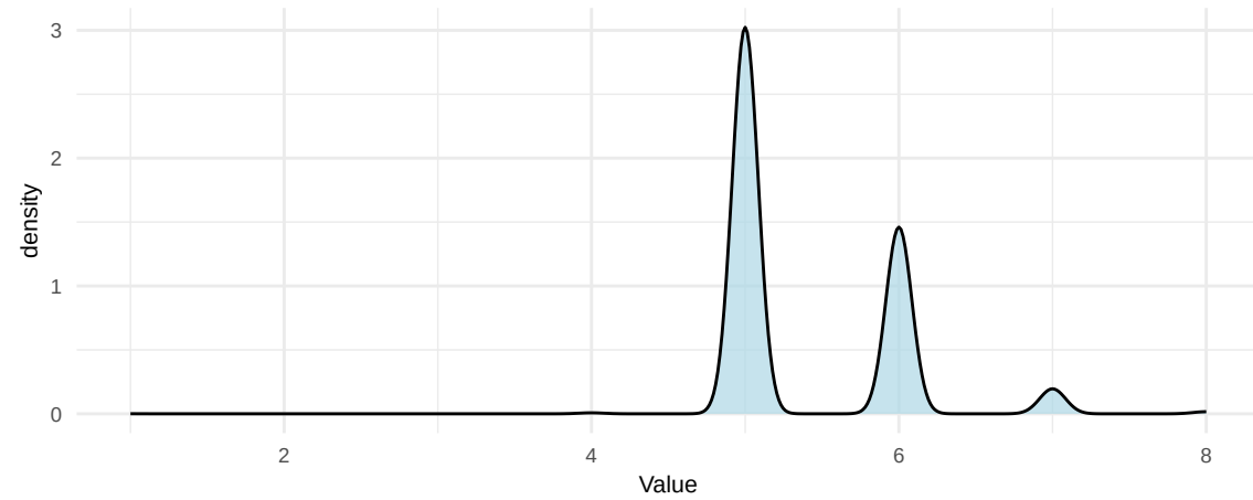
K death Density
