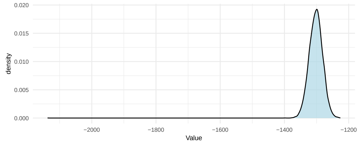
K birth Density
