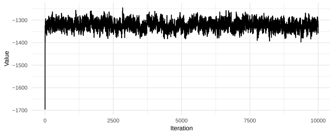
K birth Trace
