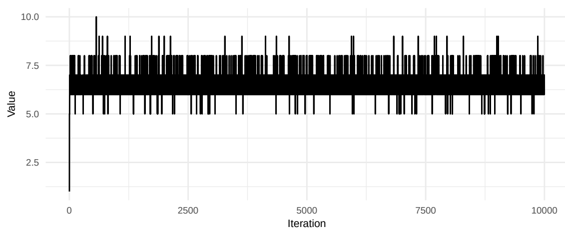
K death Trace
