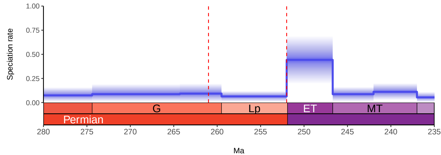
All Reptilia Model 7: BDNN MCMC by Stages with Isotopic Predictors
