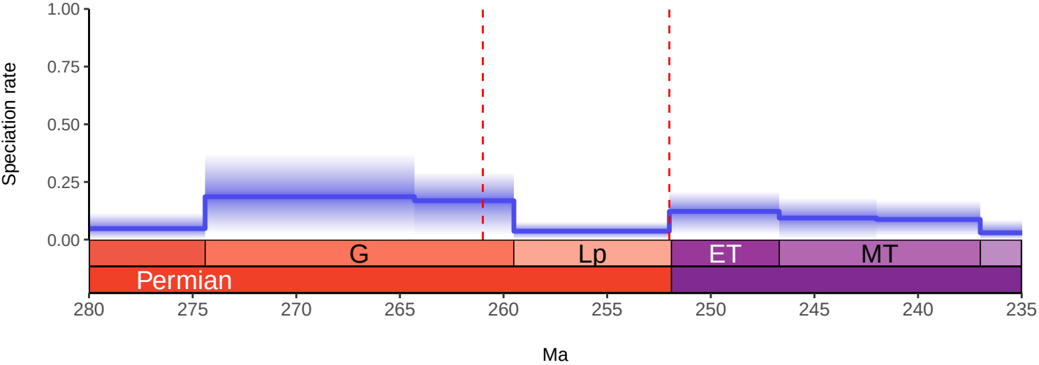
Synapsida Model 7: BDNN MCMC by Stages with Isotopic Predictors
