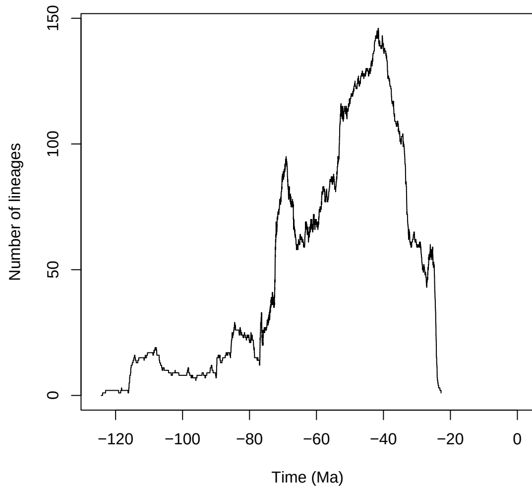
Diversity trajectory
