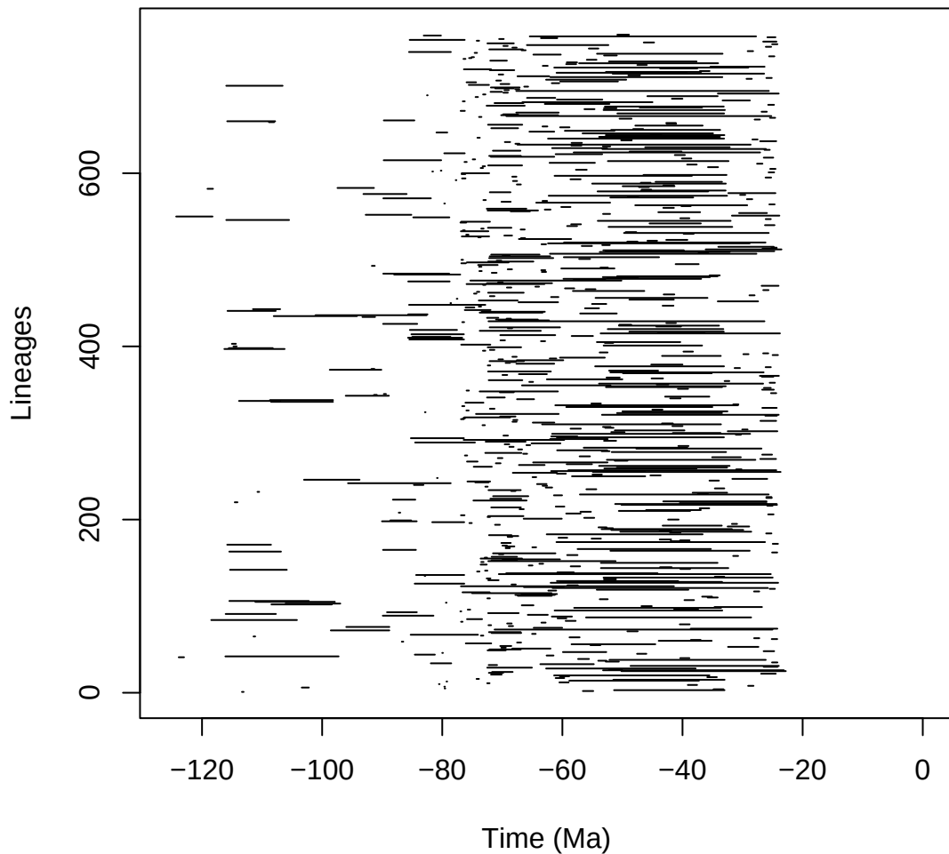
reptilia_pyrate_2_G_COVhp_BDS_mcmc
