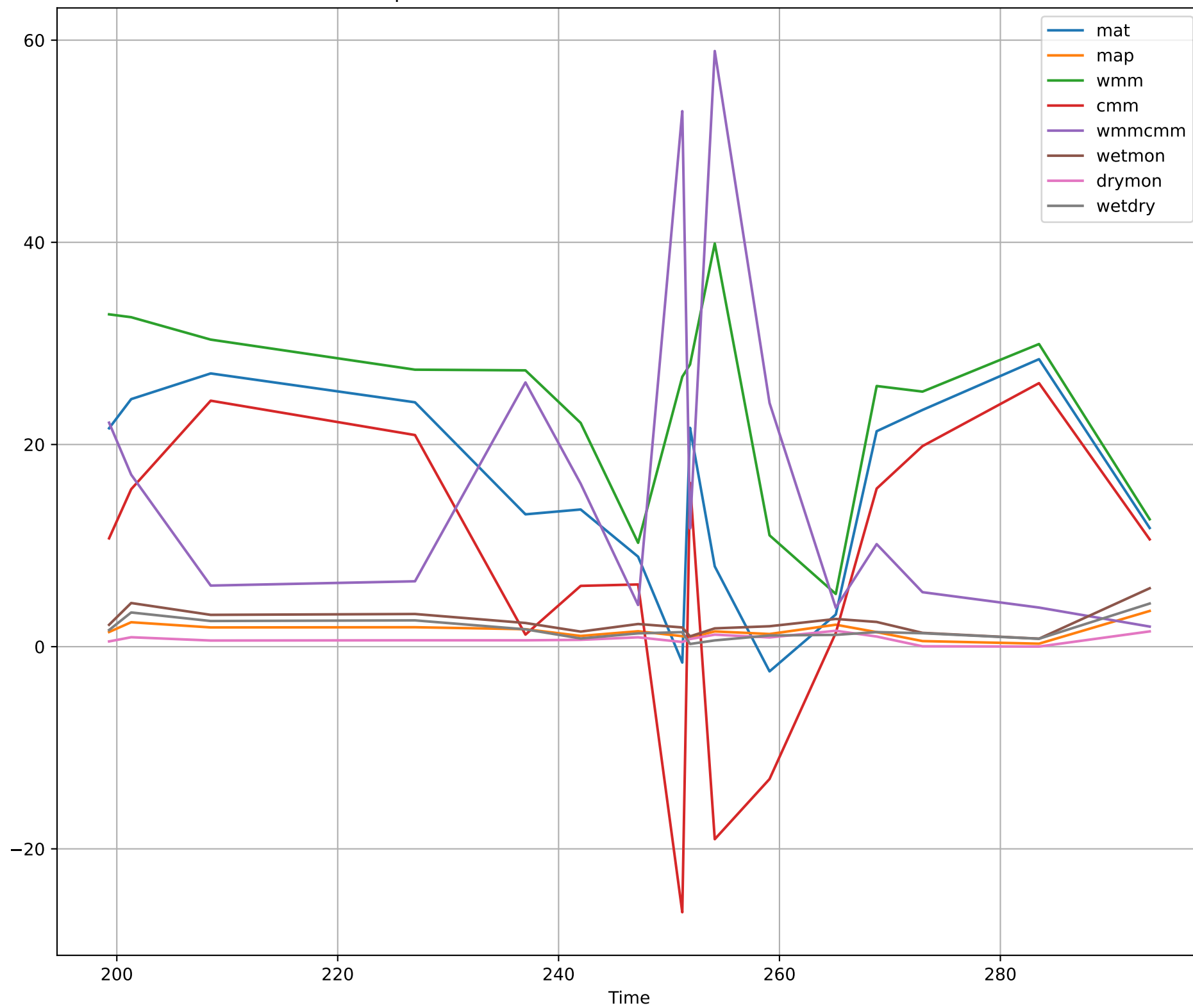
Reptilia Raw Climactic BRIDGE Variables over Time
