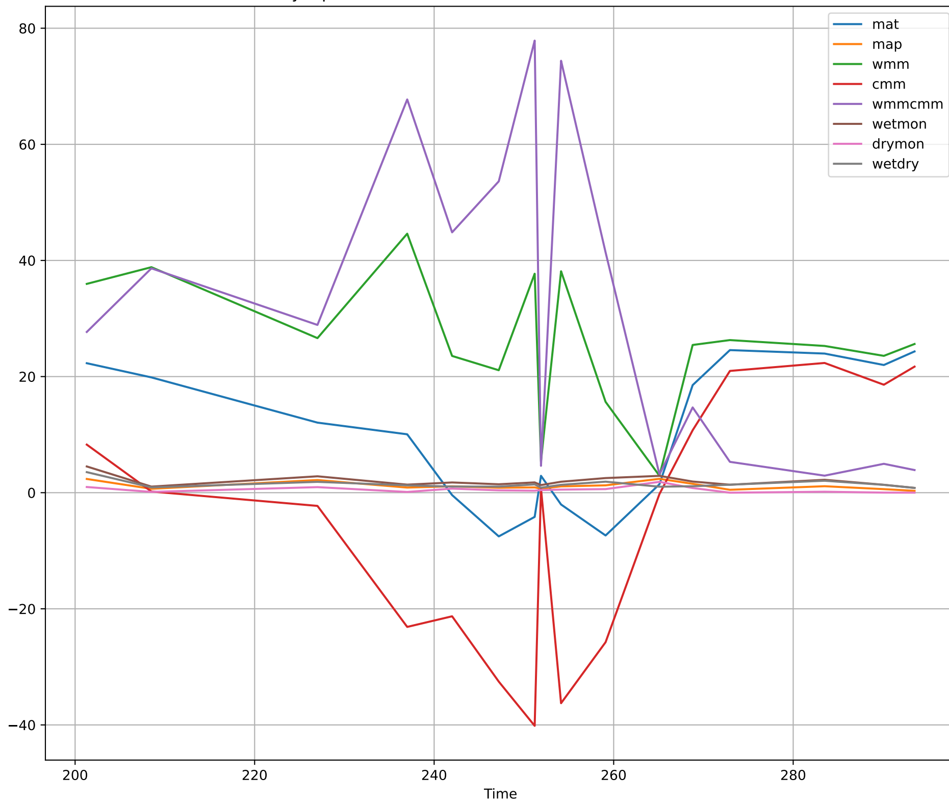
Synapsida Raw Climactic BRIDGE Variables over Time
