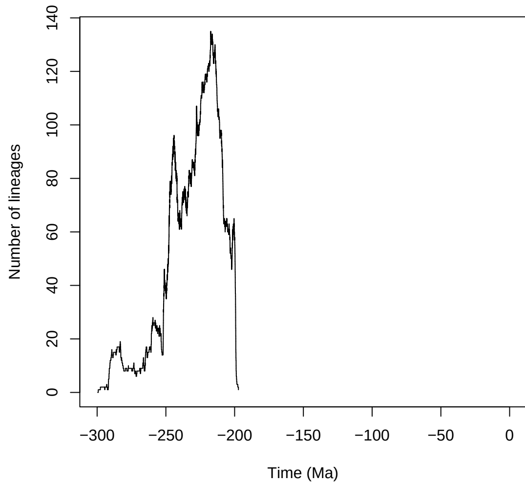
Diversity trajectory
