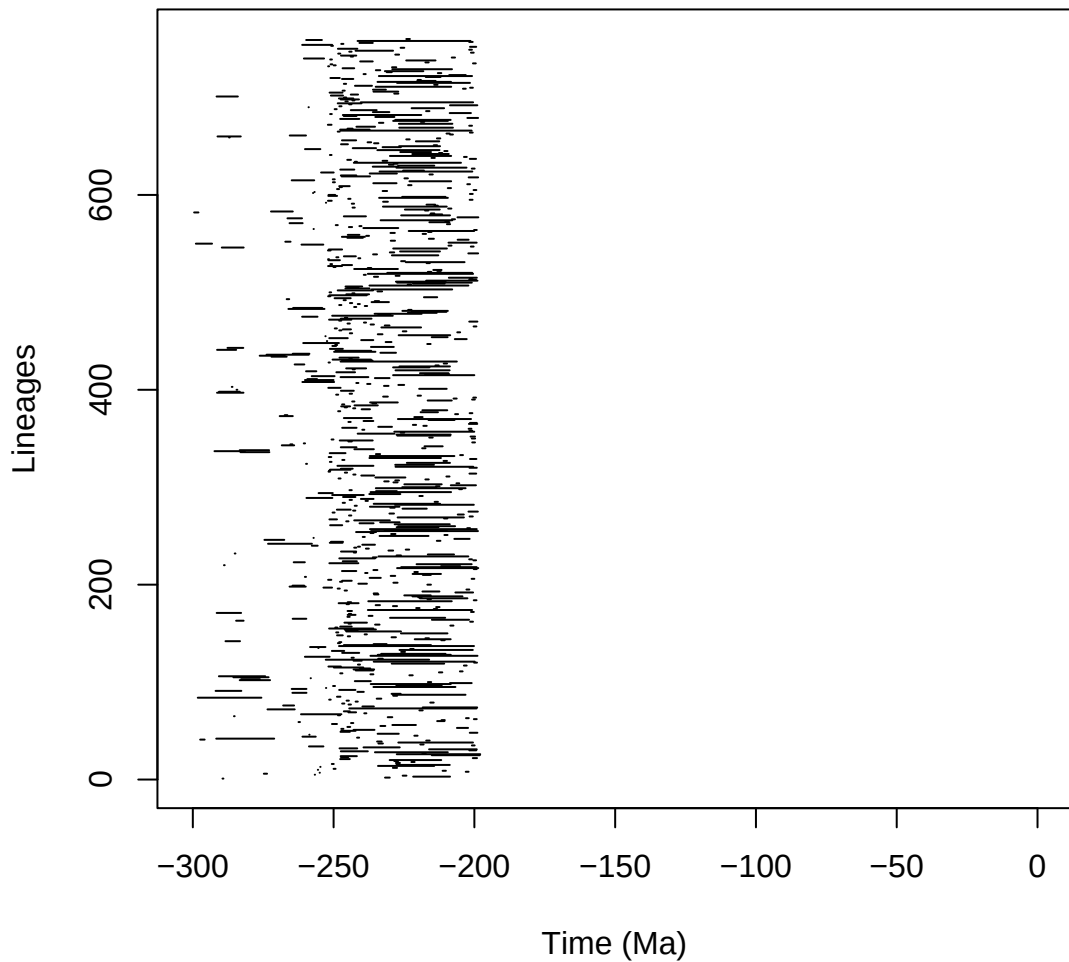
reptilia_pyrate_4_B_mcmc_G_COVhp_BD1-1_mcmc
