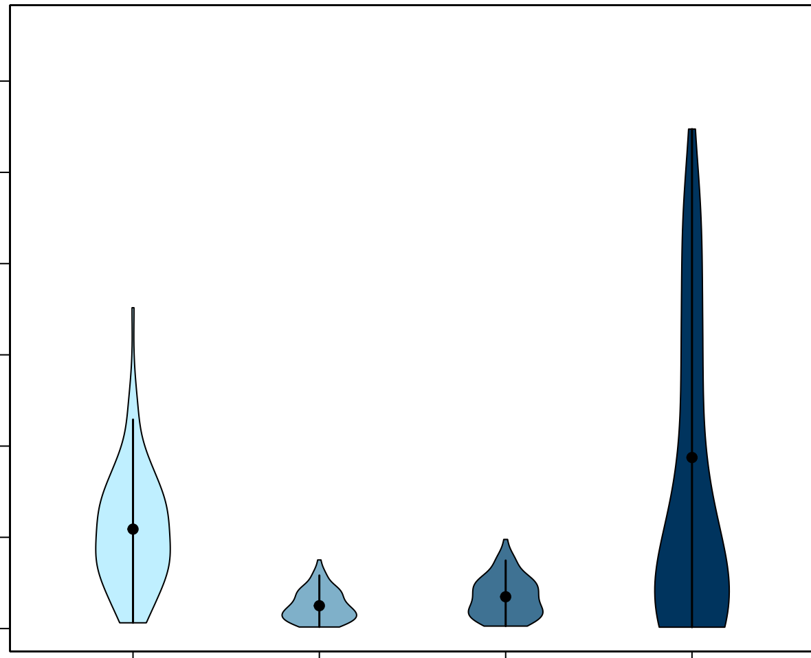
biome
