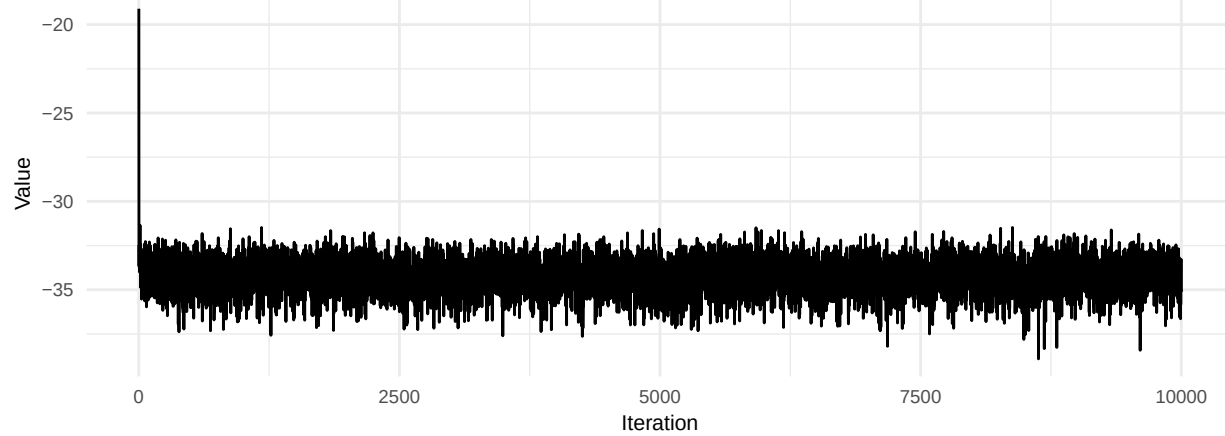
PP lik Trace
