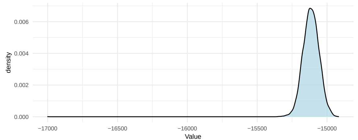
Prior Density
