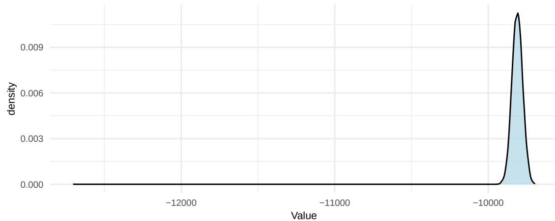
Prior Density
