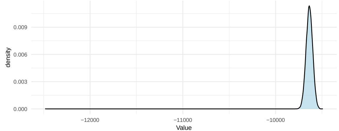
Prior Density
