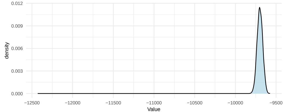
Prior Density
