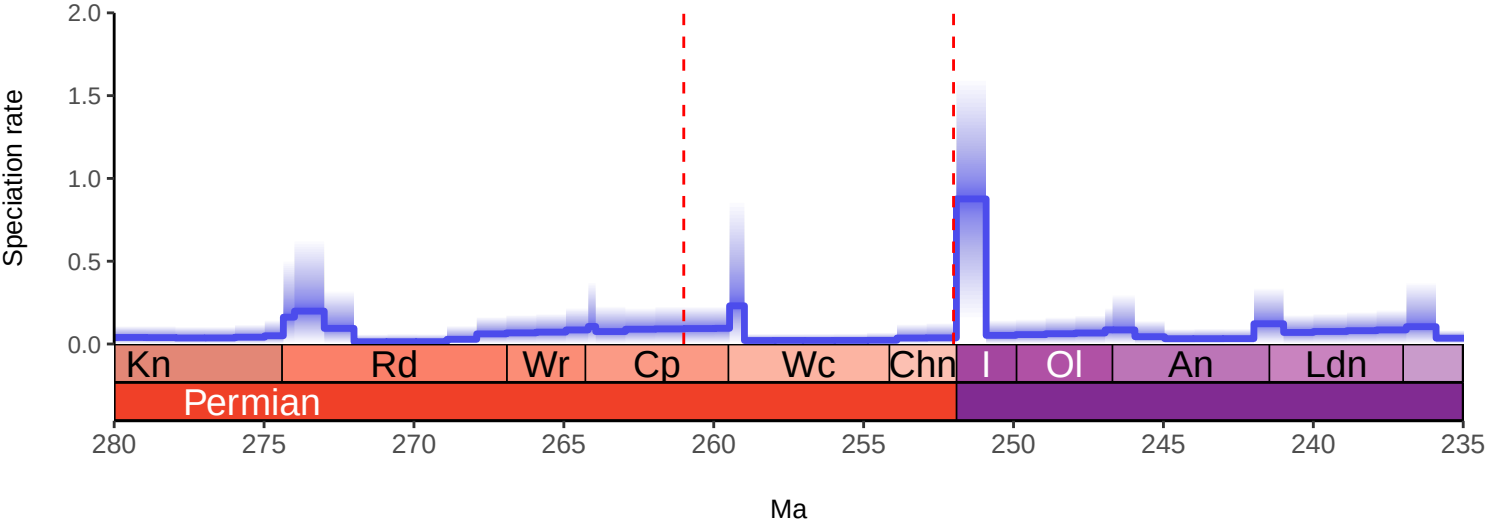
Terrestrial Reptilia Model 9: BDNN MCMC by 1Myr with 1Myr BRIDGE Predictors
