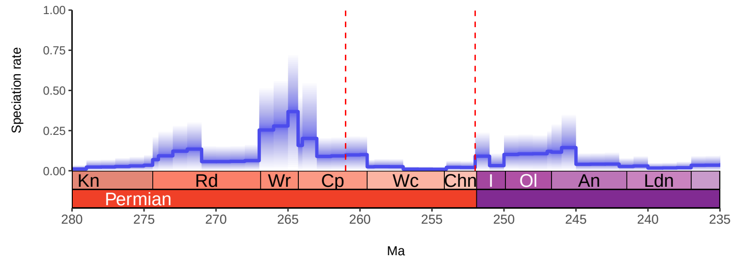
Synapsida Model 9 NEW Interpolation: BDNN MCMC by 1Myr with 1Myr BRIDGE Pred
