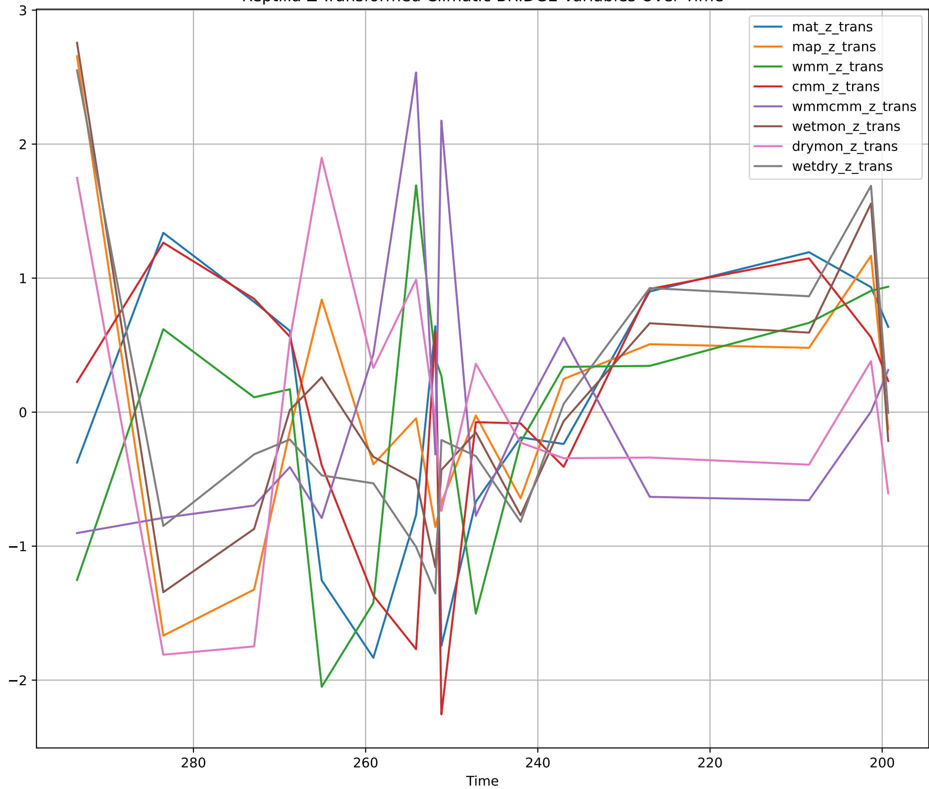
Reptilia Z-Transformed Climatic BRIDGE Variables Over Time
