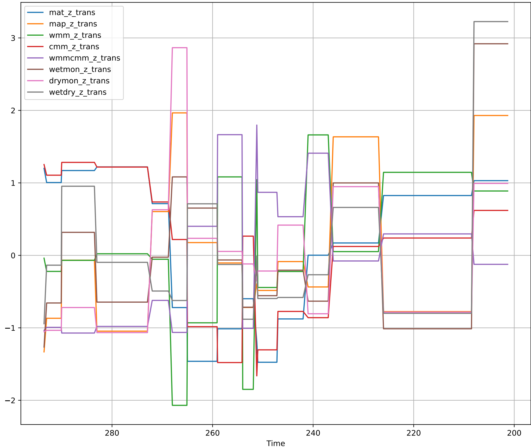
Synapsida Z-Transformed Climatic BRIDGE (1Myr Extension) Variables over Time
