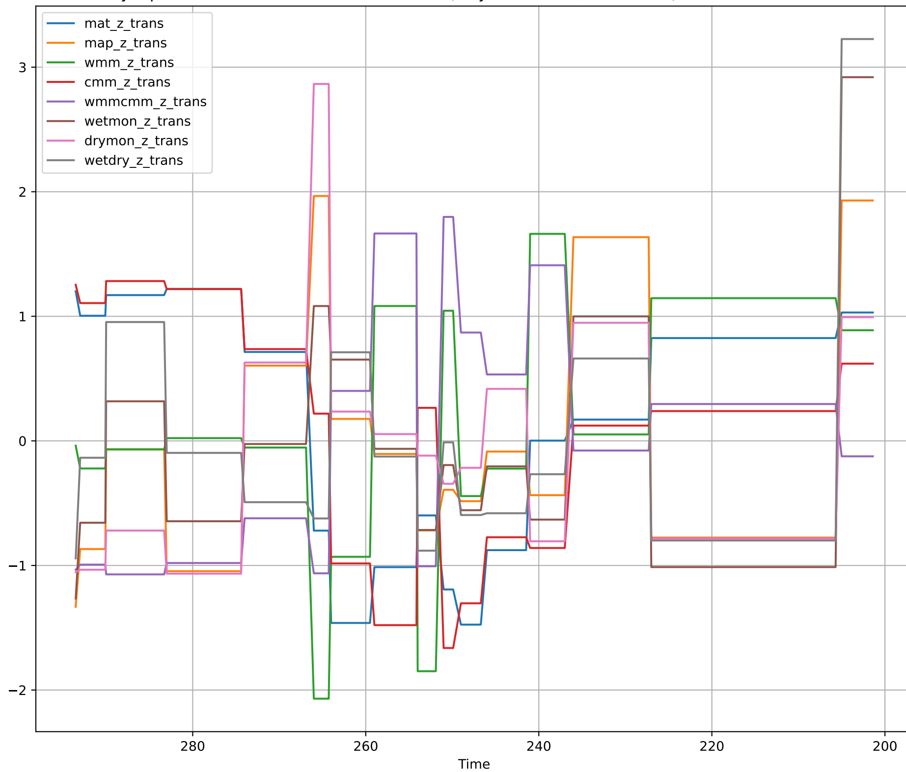
Synapsida Z-Transformed Climatic BRIDGE (1Myr Extension, New Dates) Variables over Time
