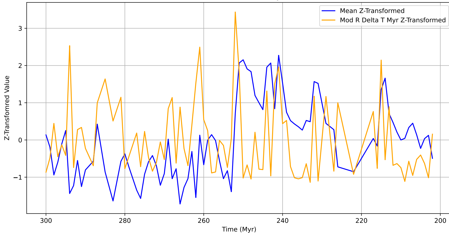
Z-Transformed Mean and Mod R Delta T Myr Over Time BY 1MYR
