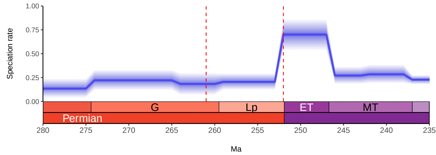
Terrestrial Reptilia Model 1: MCMC by Stages with No Predictors
