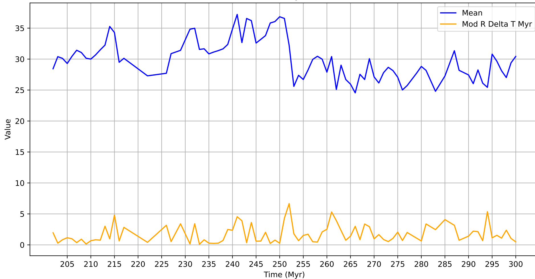
Mean and Mod R Delta T Myr Over Time BY 1MYR
