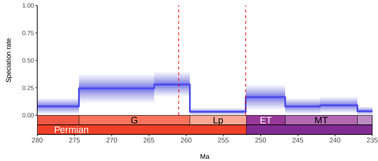
Synapsida Model 7: BDNN MCMC by Stages with Isotopic Predictors by G-L Stages
