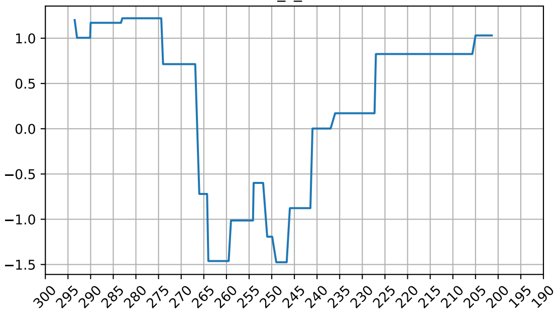
wmm_z_trans
