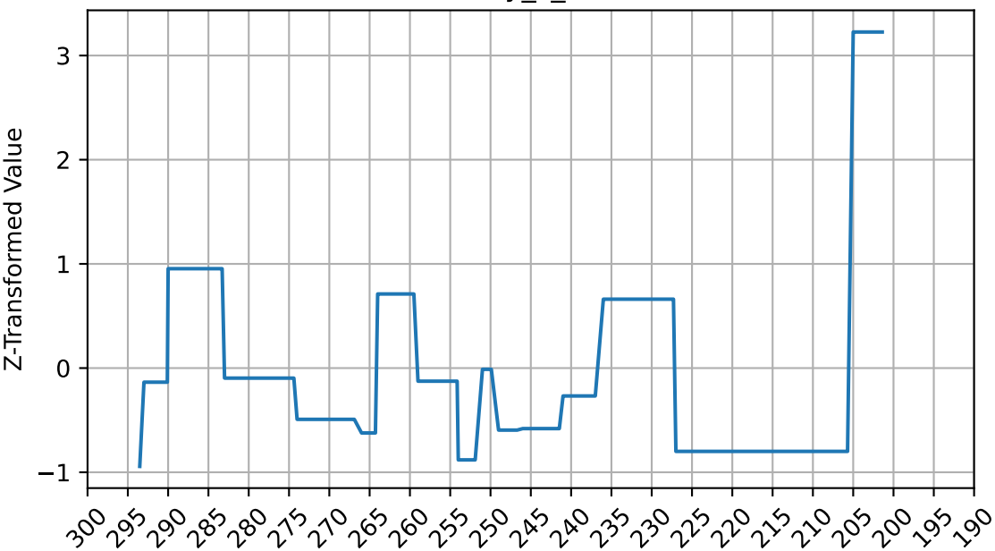
wetdry_z_trans
