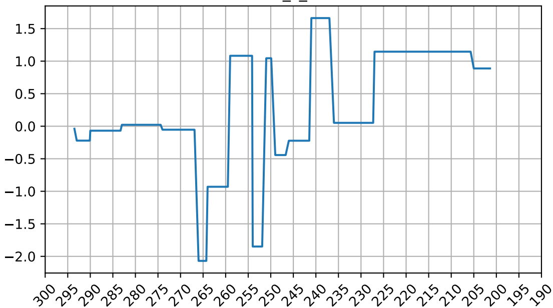
wmmcmm_z_trans
