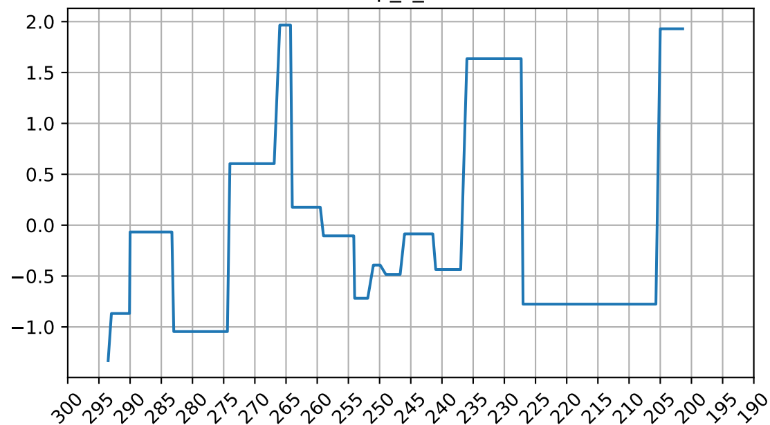
cmm_z_trans
