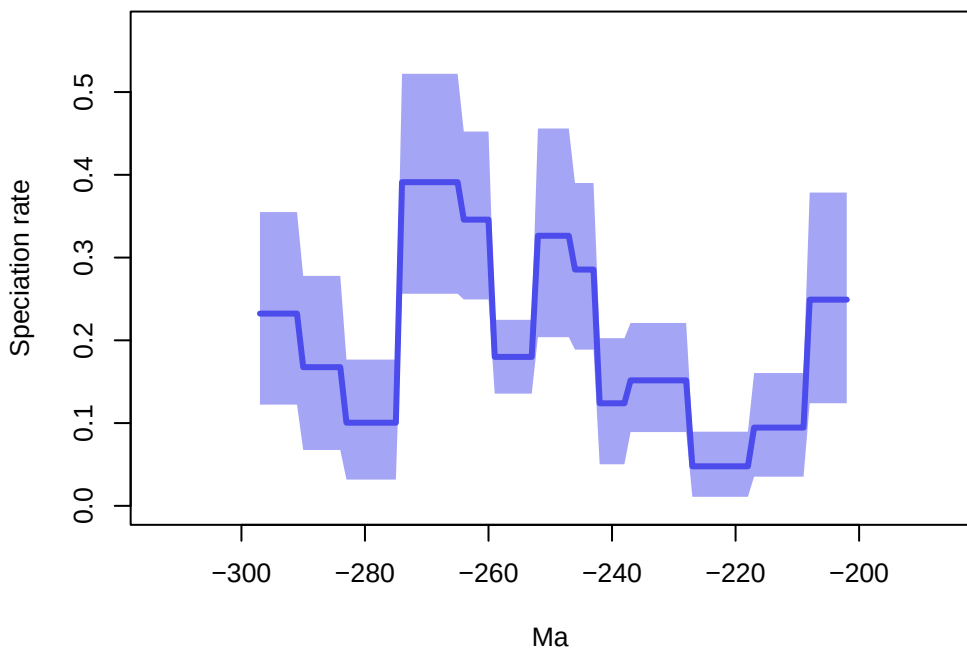
Synapsida: MCMC By Stages No Preds
