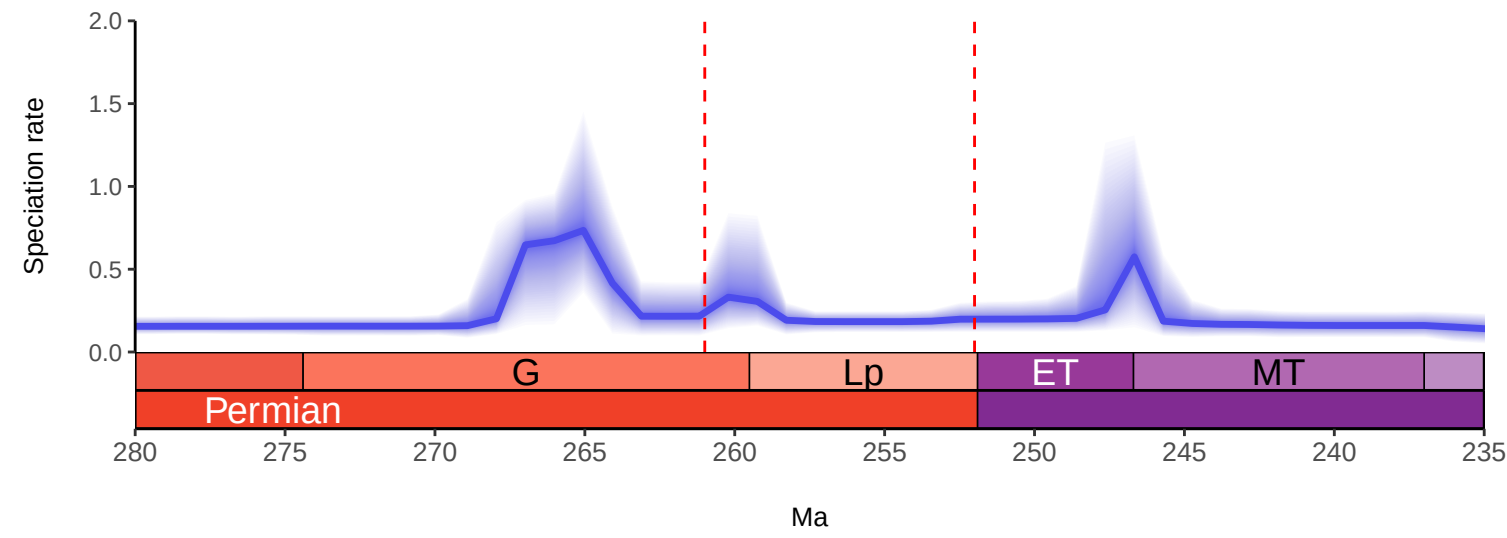
Synapsida Models 2 & 5: RJMCMC by 1Myr with No Predictors
