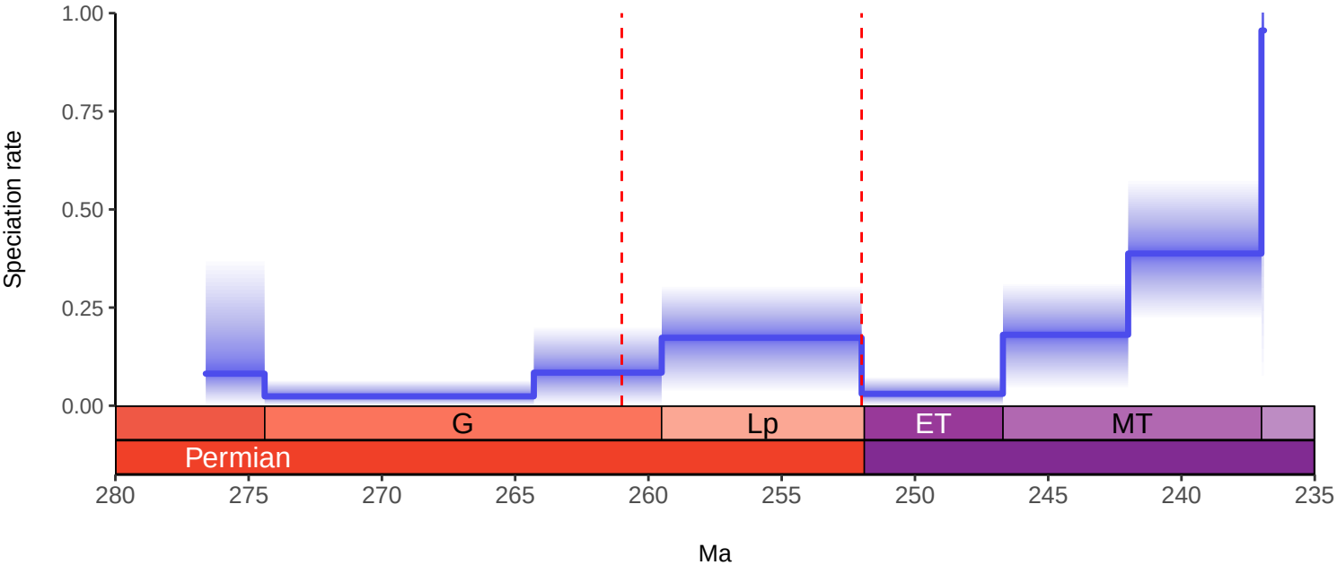
Synapsida Model 4: MCMC by Stages with BRIDGE Predictors
