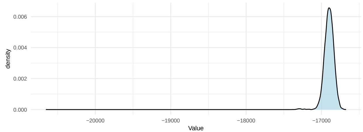
Prior Density
