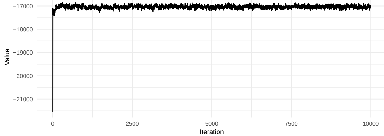
Prior Trace
