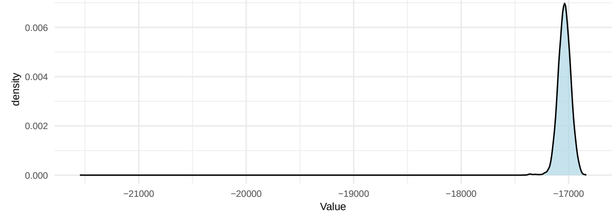
Prior Density
