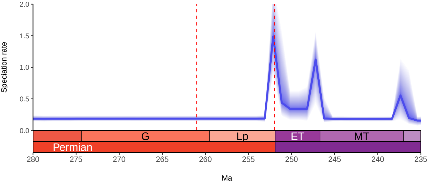
All Reptilia Model 5: RJMCMC by 1 Myr with No Predictors
