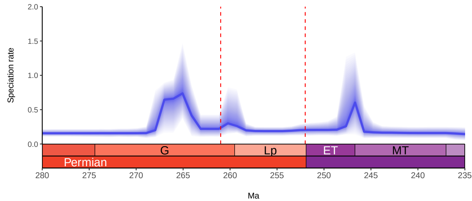
Synapsida Models 2 & 5: RJMCMC by 1 Myr with No Predictors
