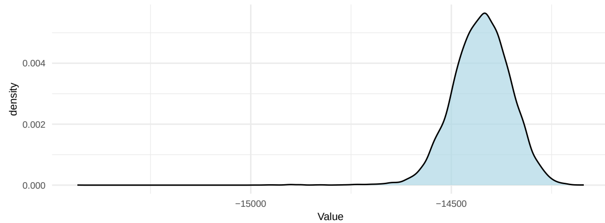
Prior Density
