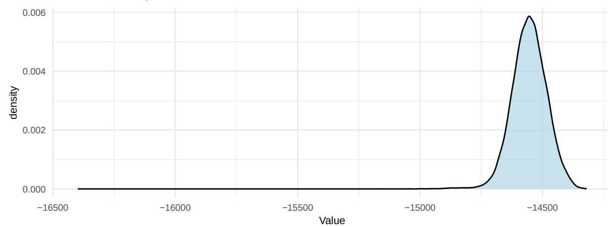
Prior Density
