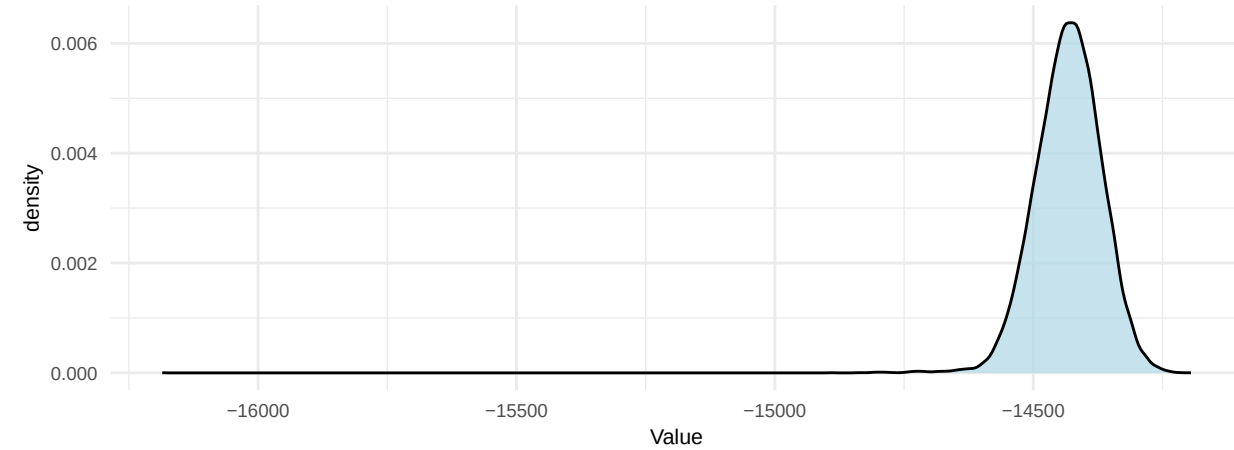
Prior Density
