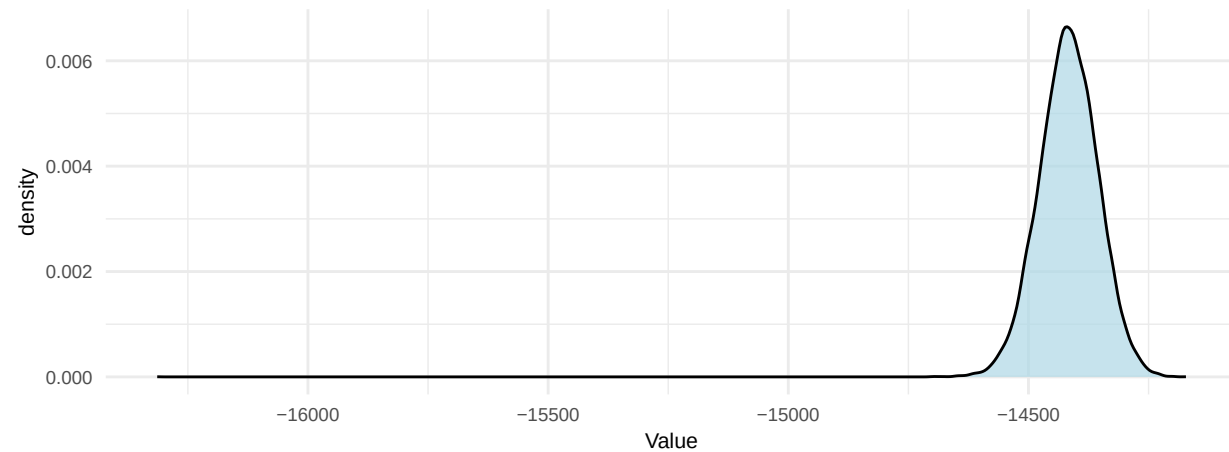
Prior Density
