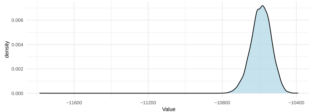
Prior Density
