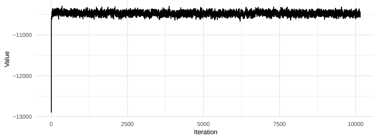
Prior Trace
