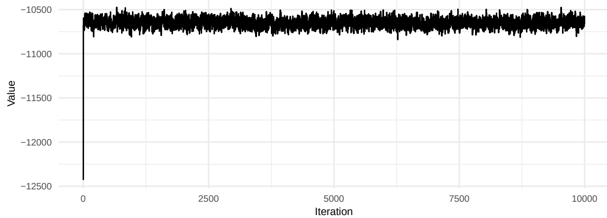
Prior Trace
