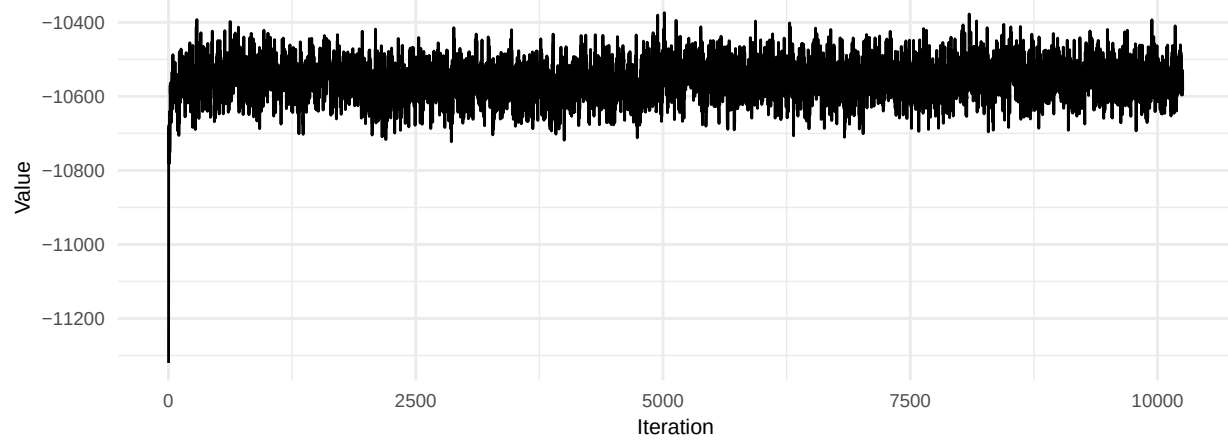
Prior Trace
