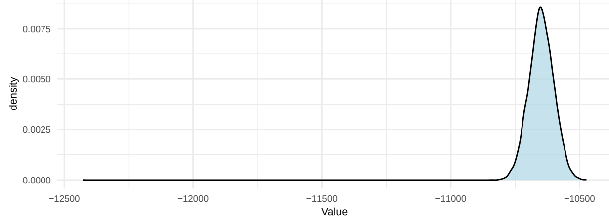
Prior Density
