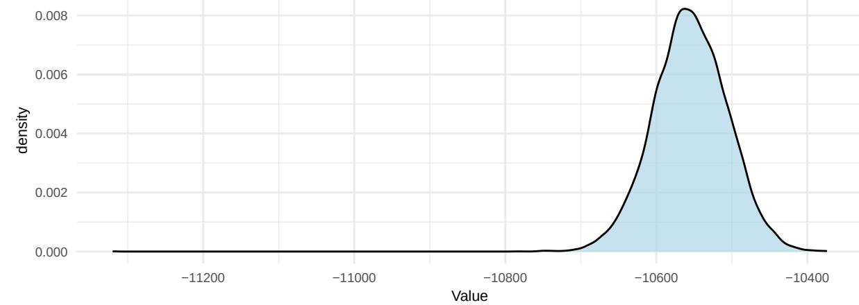
Prior Density
