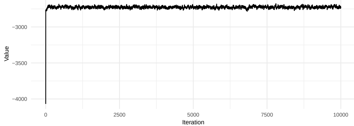
BD lik Trace
