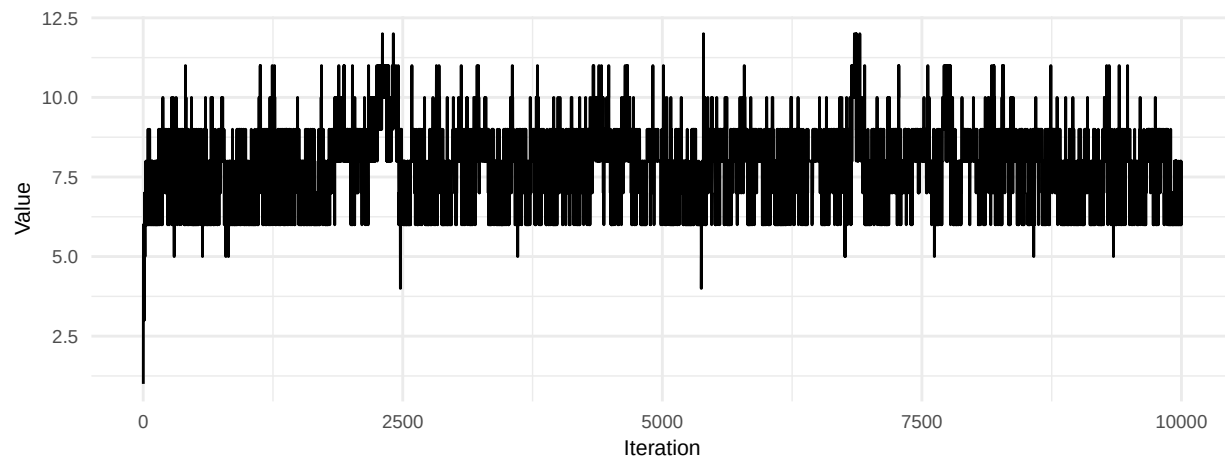
K death Trace
