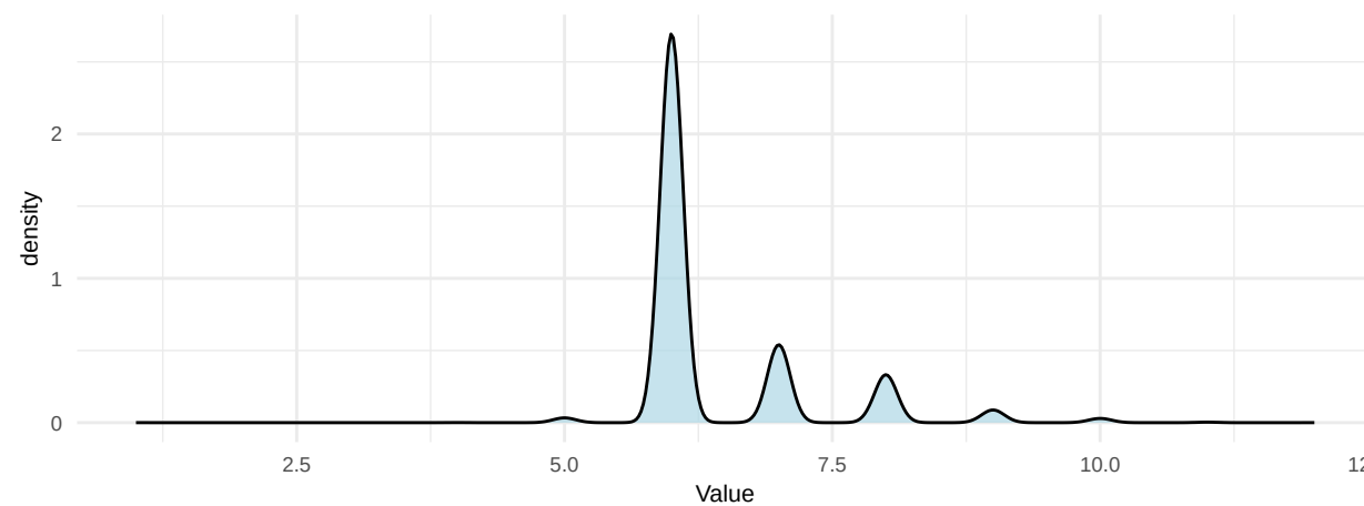
K death Density
