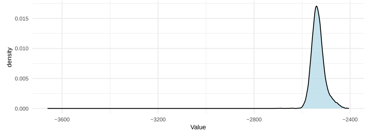
K birth Density
