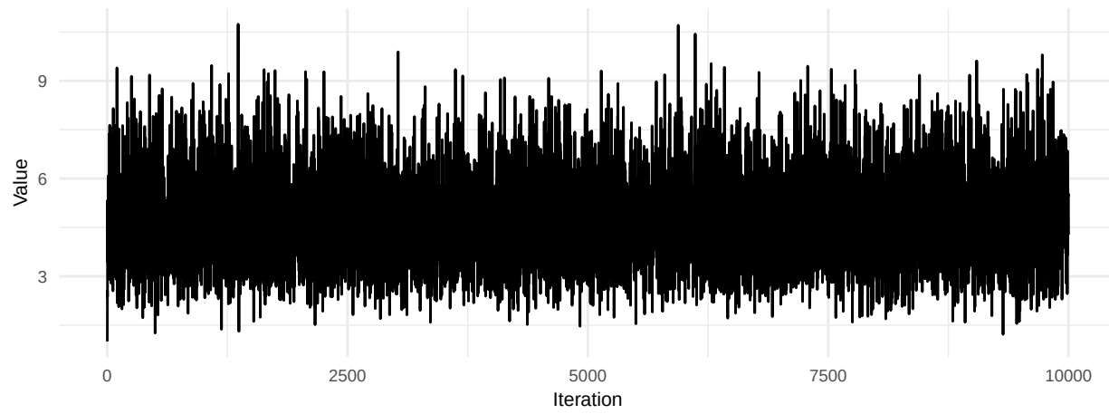
RJ hp Trace
