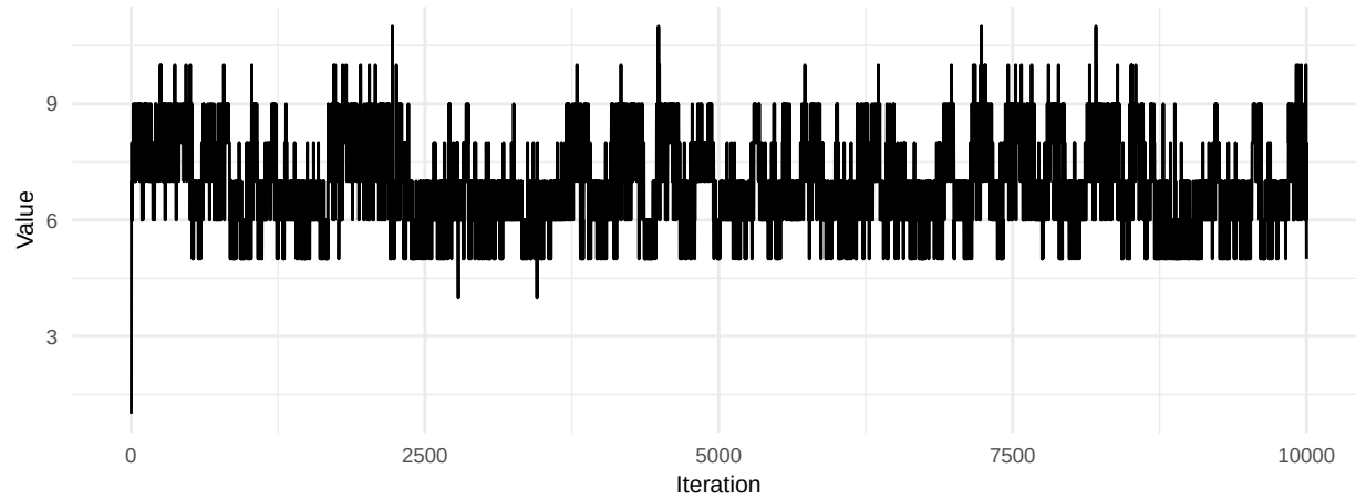
K death Trace
