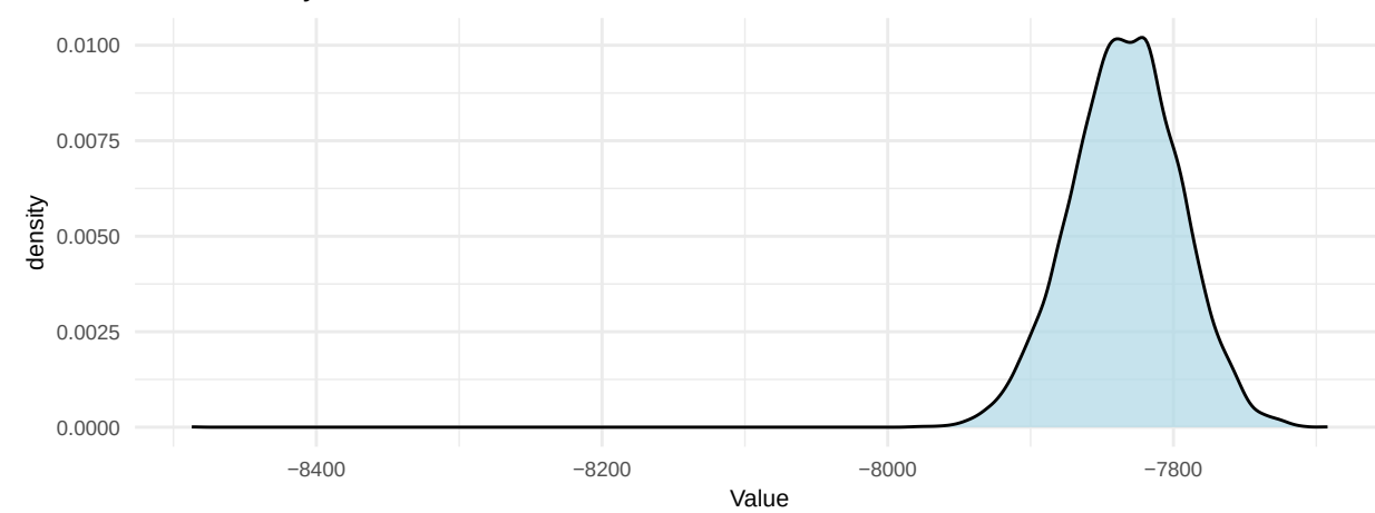
PP lik Density
