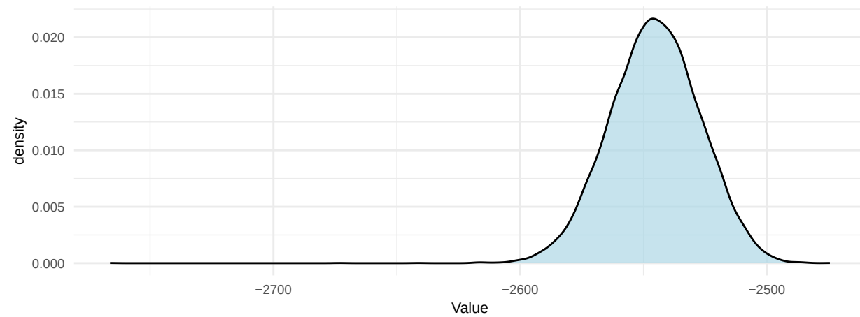
K birth Density
