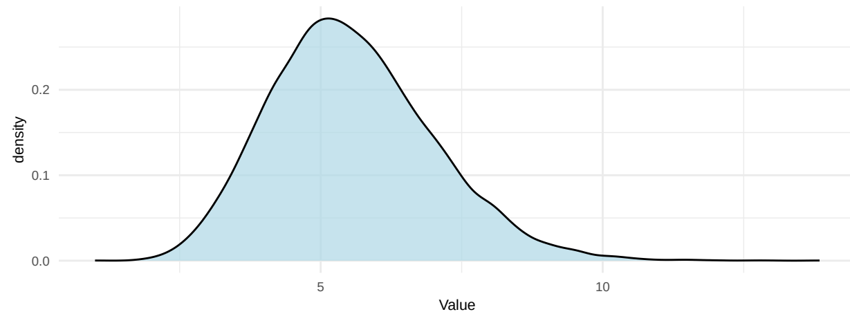
RJ hp Density
