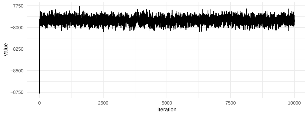
PP lik Trace
