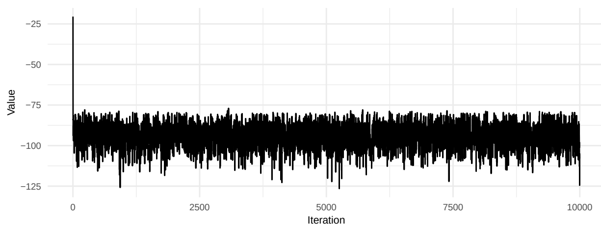
PP lik Trace
