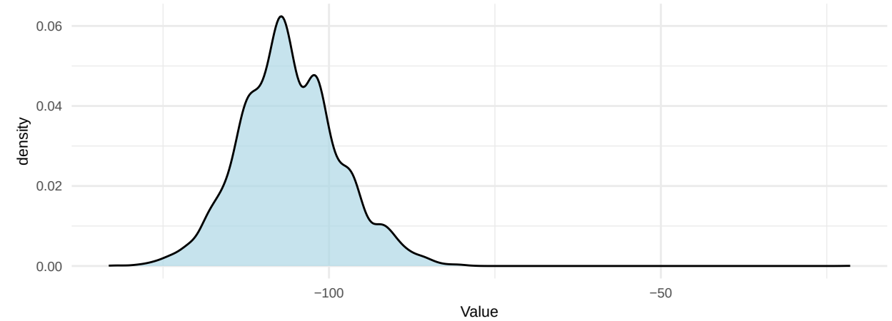
PP lik Density
