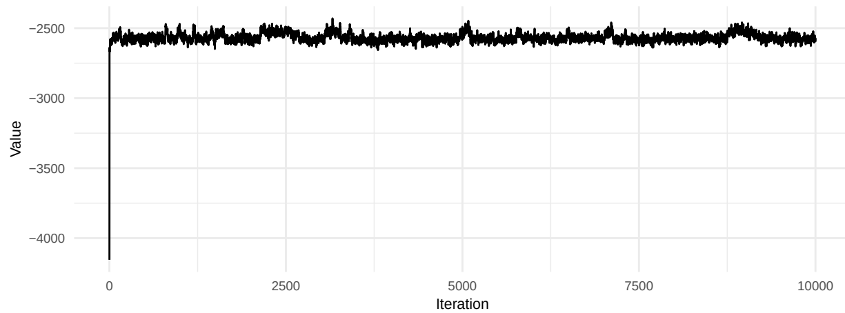
K birth Trace
