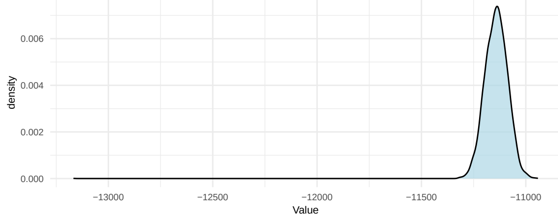
Prior Density
