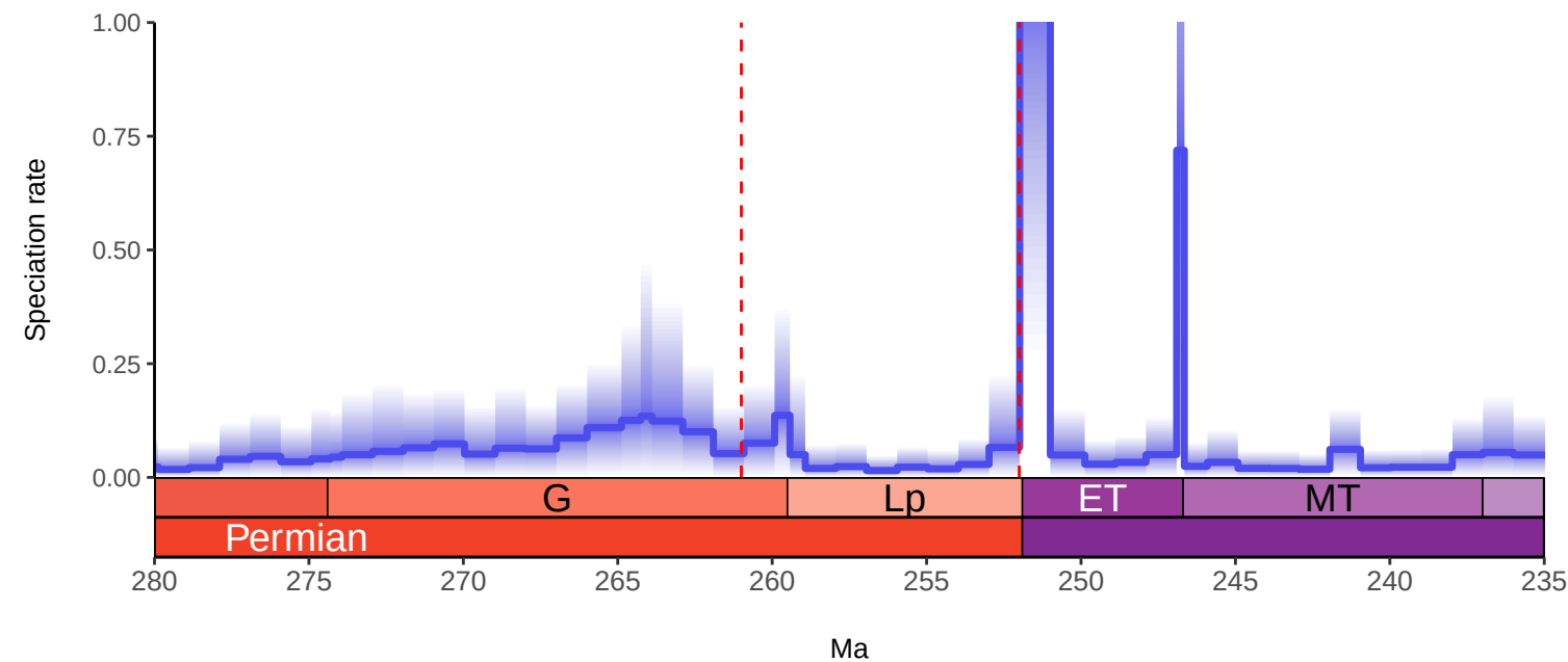
All Reptilia Model 8: BDNN MCMC by 1Myr with Isotopic and Stage Predictors
