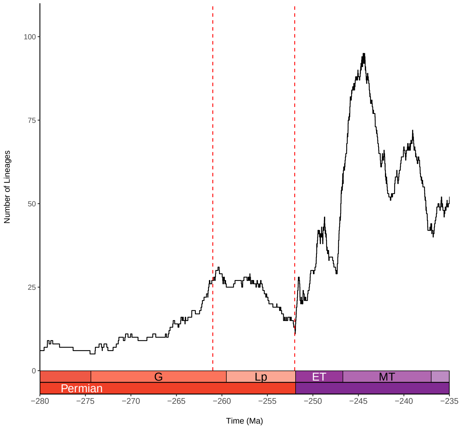
All Reptilia Model 7 Diversity Trajectory: 1Myr Isotopic Data
