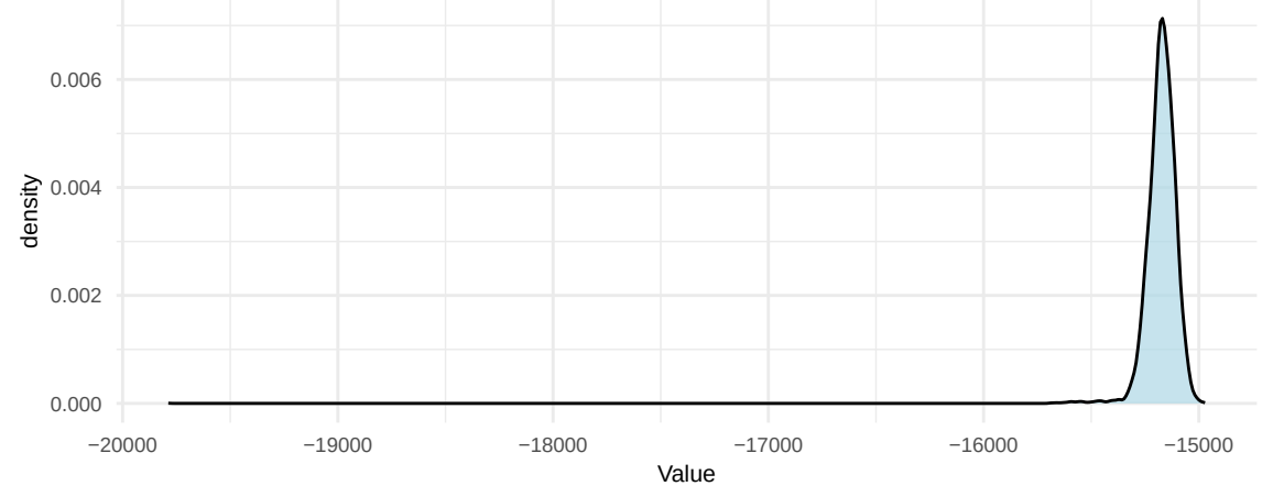
Prior Density
