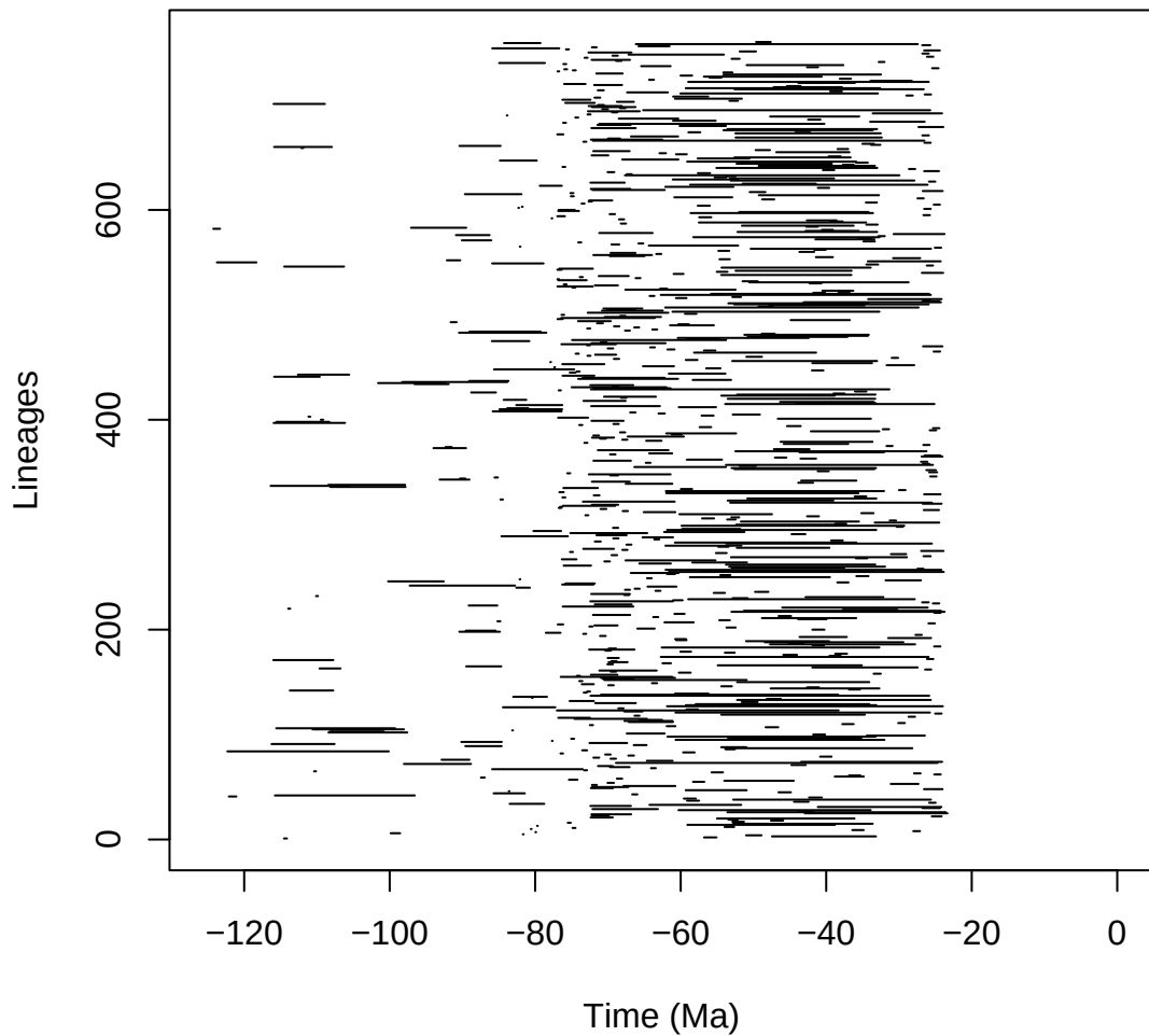
reptilia_pyrate_4_G_COVhp_BDS_mcmc
