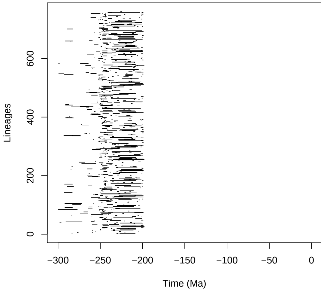
reptilia_pyrate_8_B_mcmc_G_COVhp_BD1-1_mcmc
