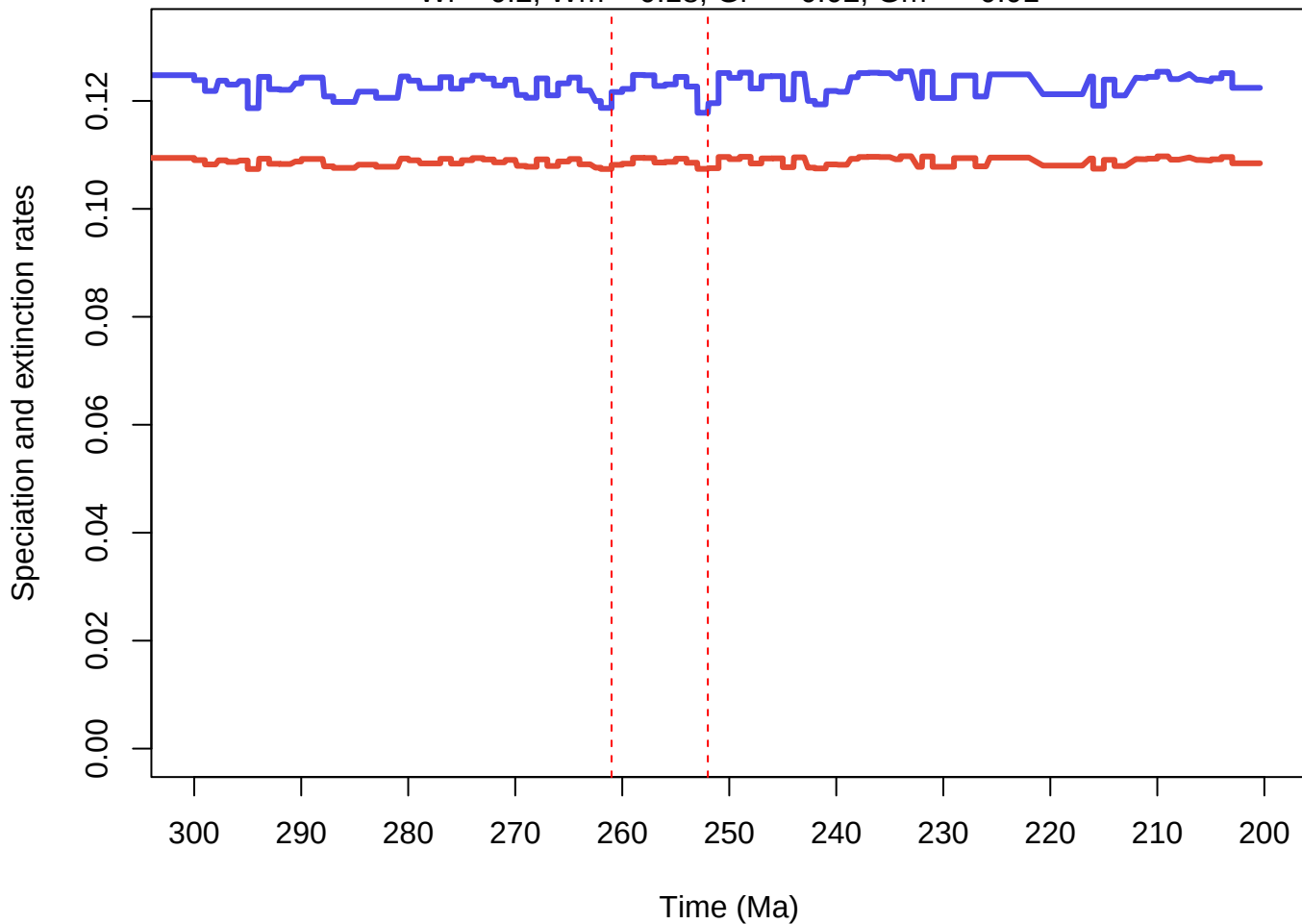
Effect of: Mod_scaled_translated
