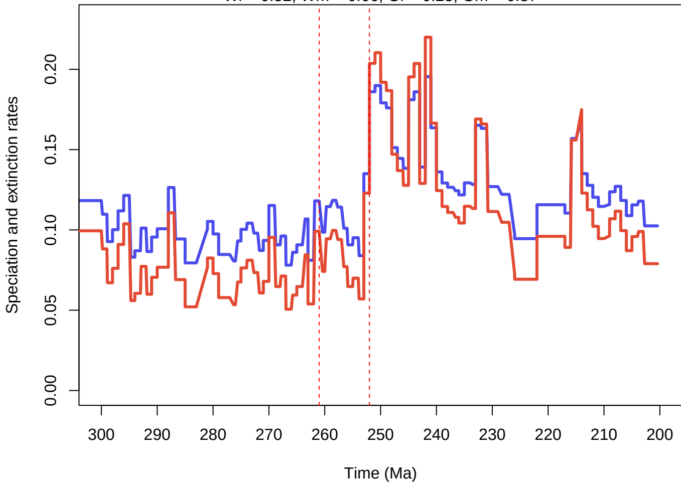
Effect of: mean_scaled_translated
