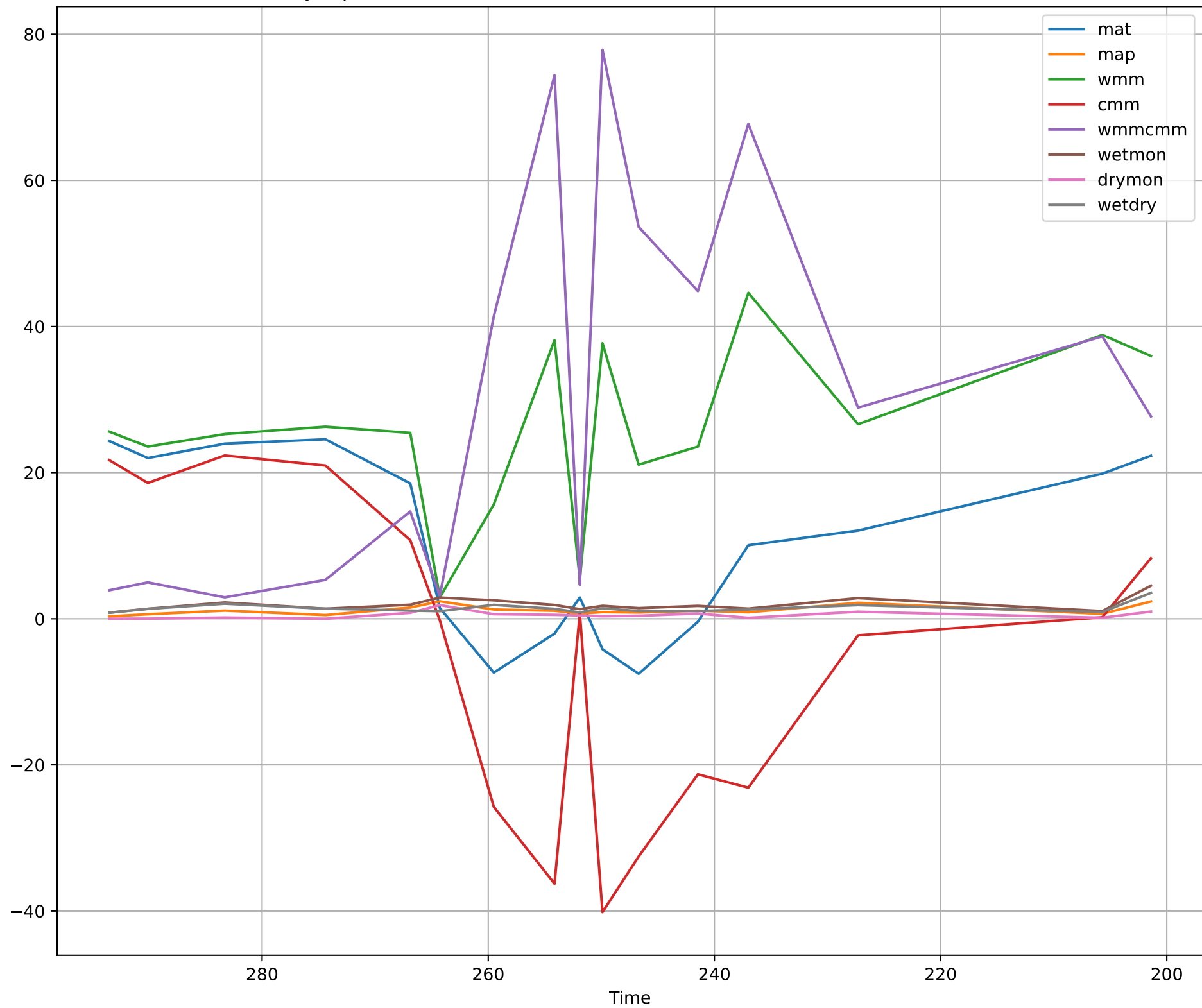
Synapsida Raw Climatic BRIDGE Variables (New Dates) Over Time
