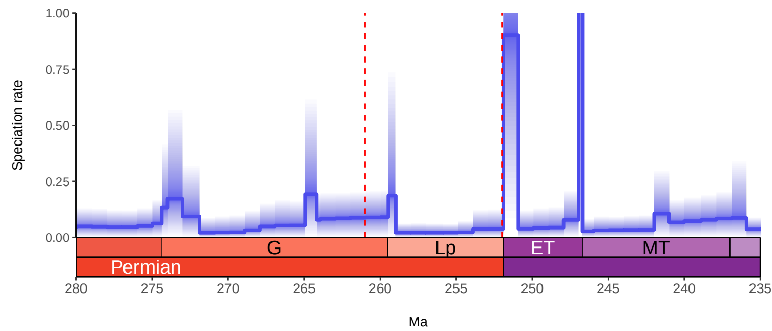
Terrestrial Reptilia Model 9: BDNN MCMC by 1Myr with BRIDGE and Stage Predictors
