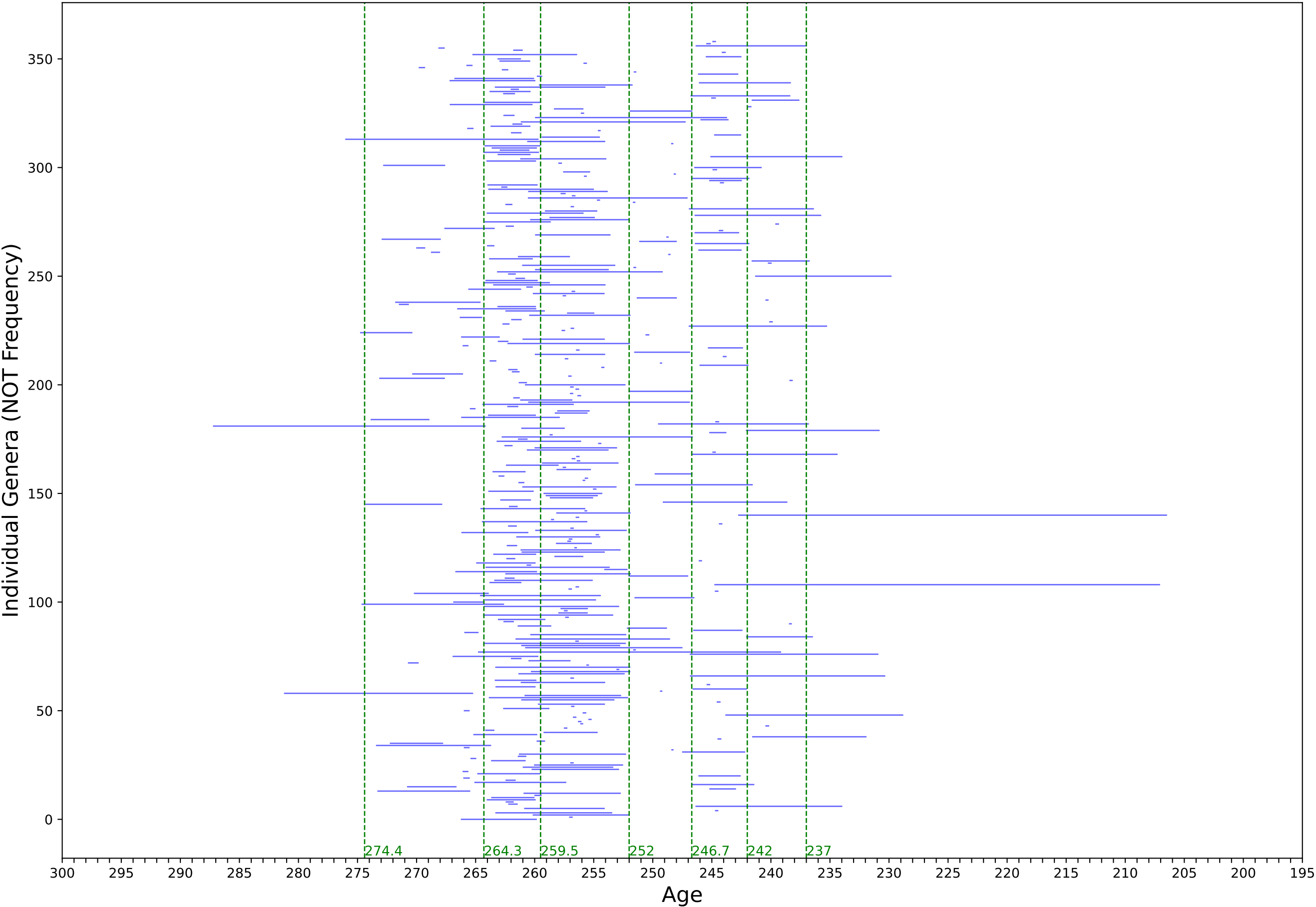
FINAL Synapsida Model 8 (Guad-Ladin Only, 237-274.4) Age Range Plot by Genus
