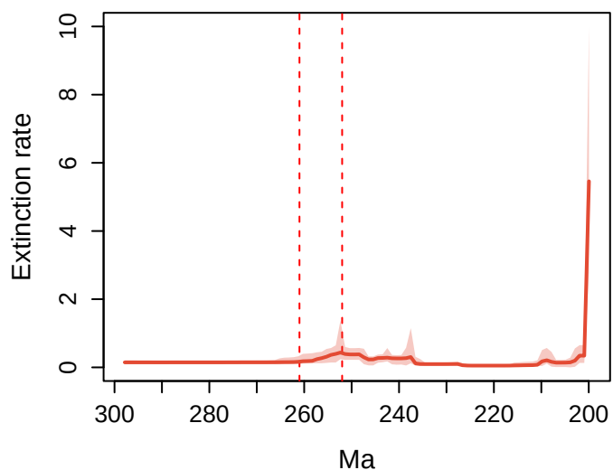
Extinction
