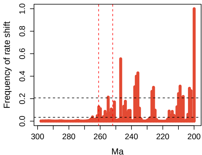
Longevity
