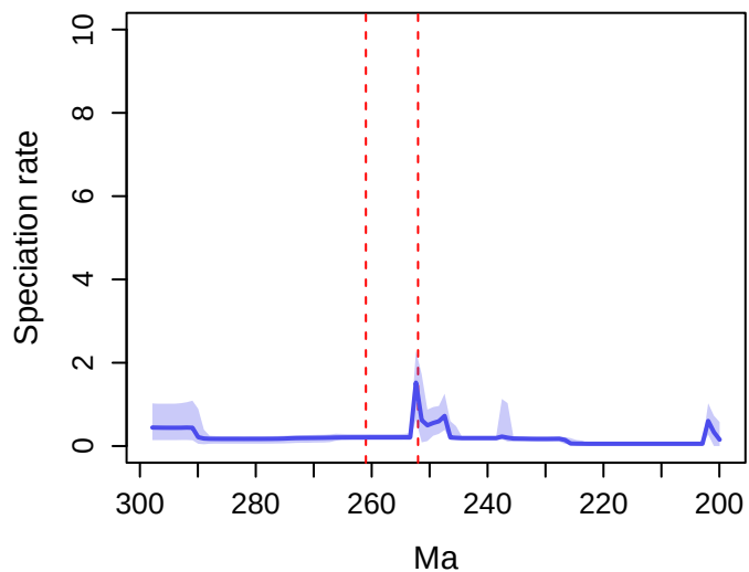
Speciation
