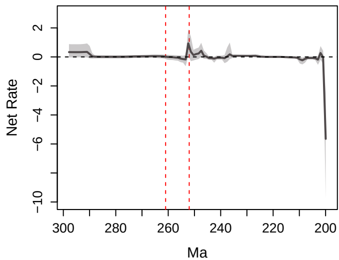
Net diversification
