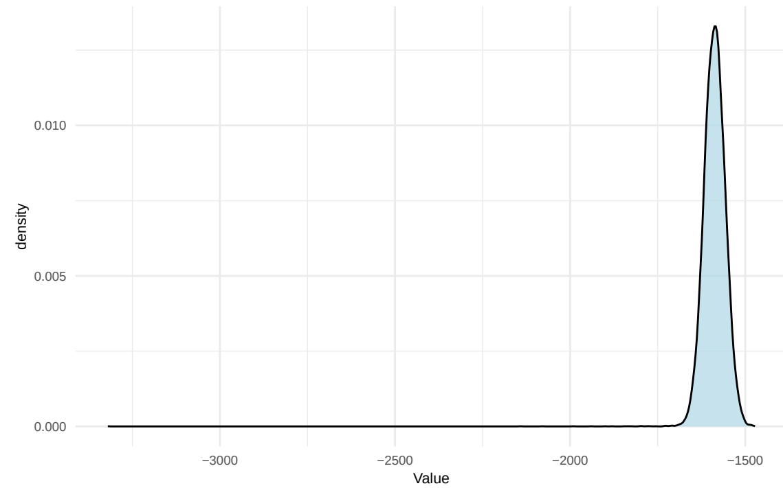
BD lik Density
