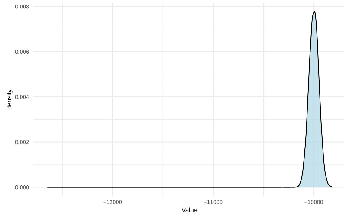
Prior Density
