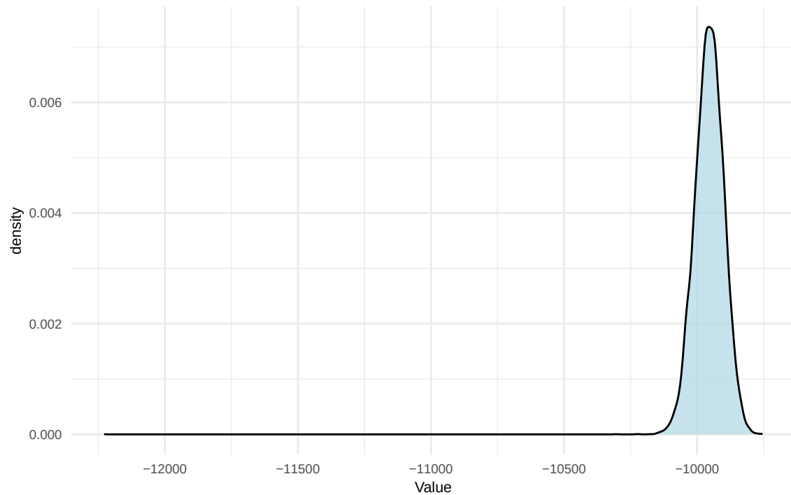
Prior Density
