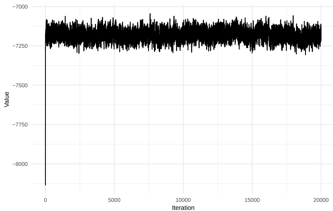
BD lik Trace
