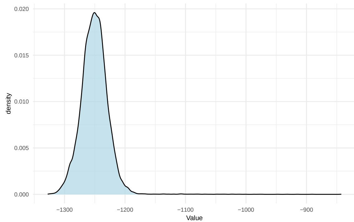
Prior Density
