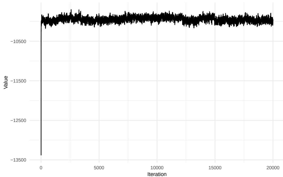
Prior Trace
