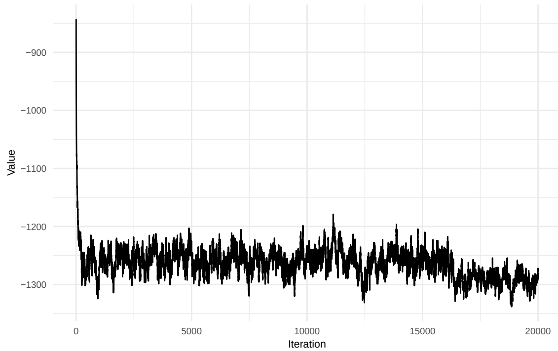
Prior Trace
