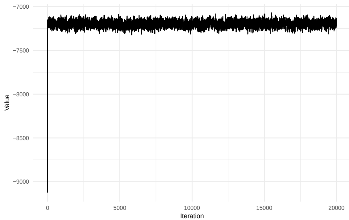
BD lik Trace
