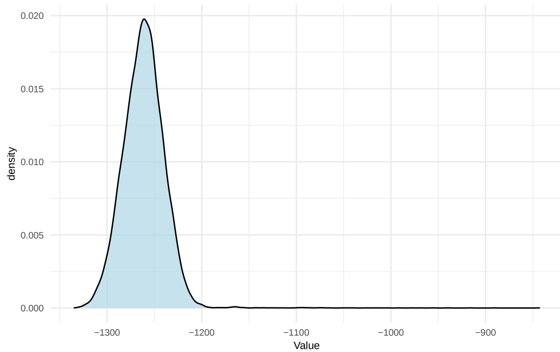
Prior Density
