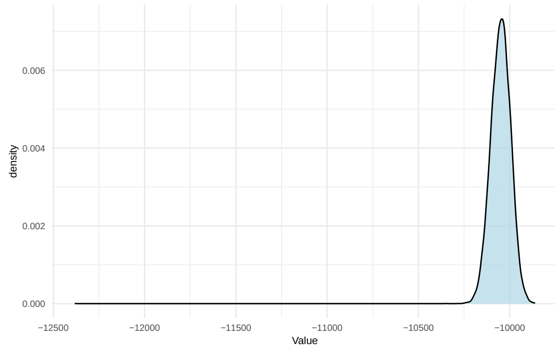
Prior Density
