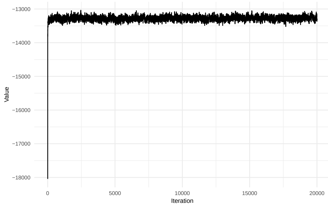
Prior Trace
