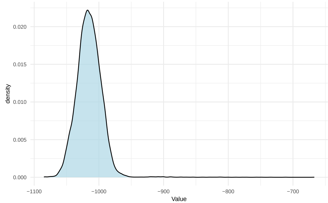
Prior Density
