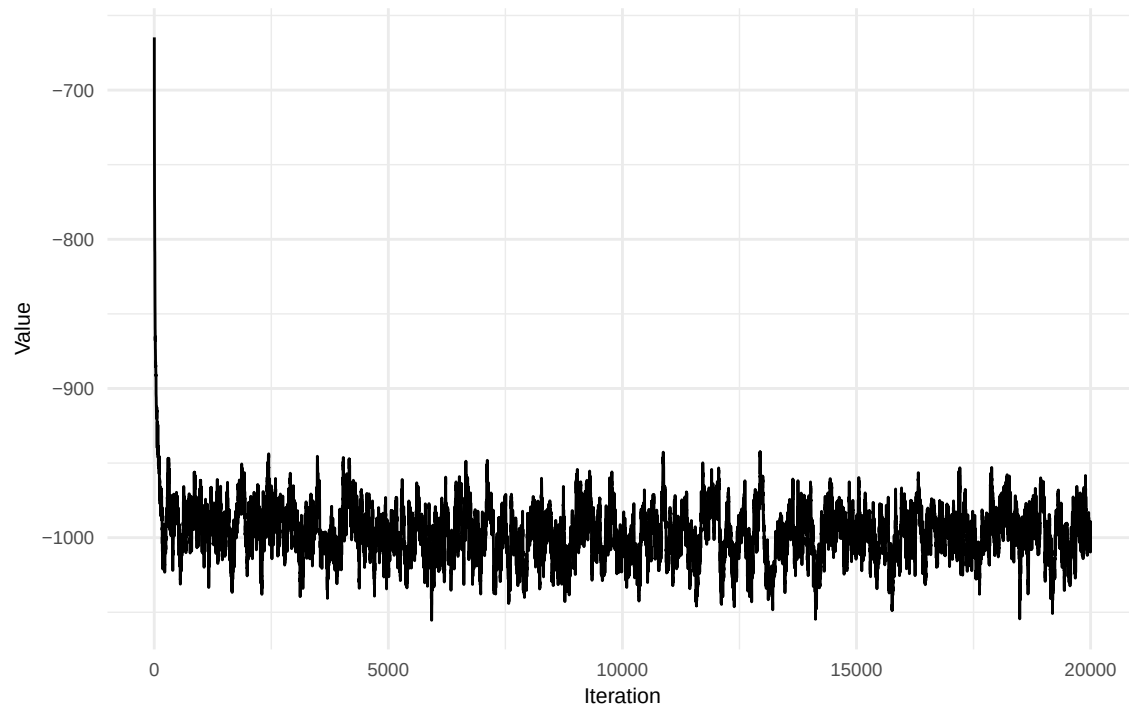
Prior Trace
