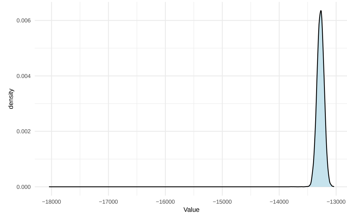
Prior Density
