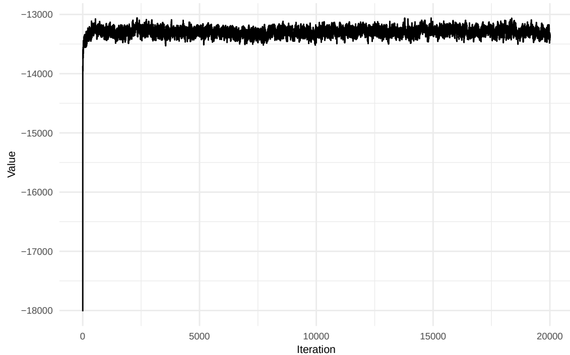
Prior Trace
