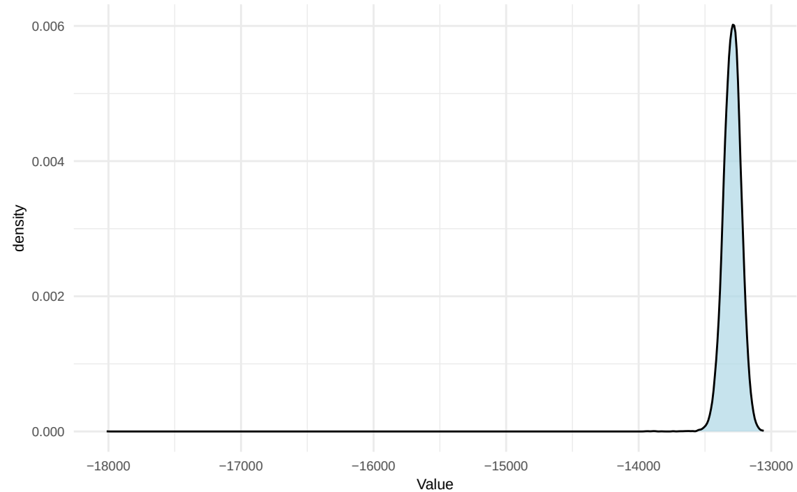
Prior Density
