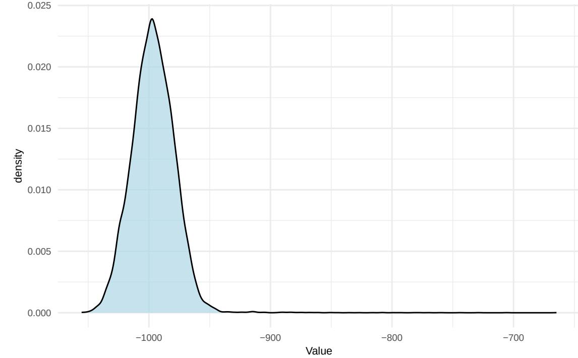
Prior Density
