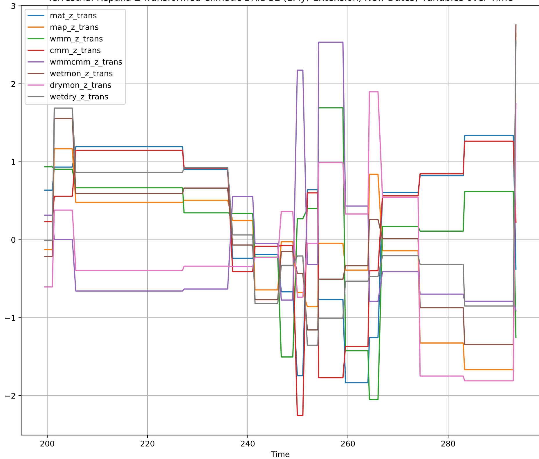
Terrestrial Reptilia Z-Transformed Climatic BRIDGE (1Myr Extension, New Dates) Variables over Time
