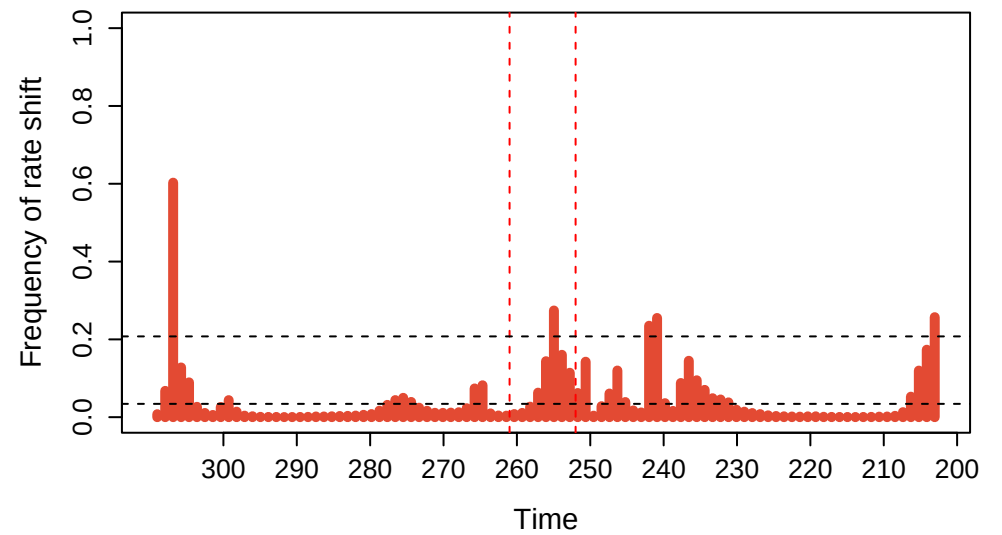
Longevity
