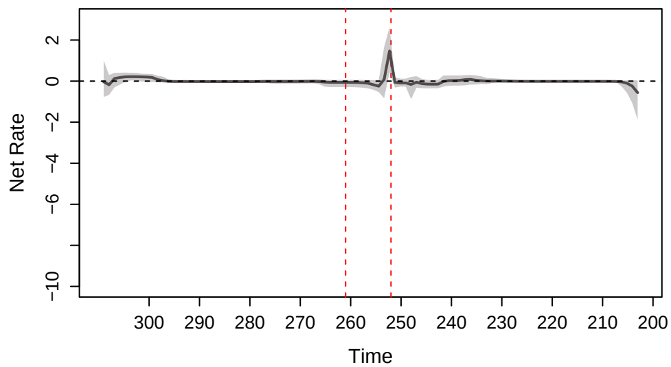
Net diversification
