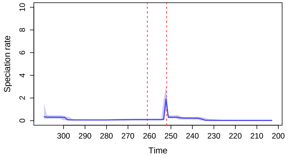
Speciation
