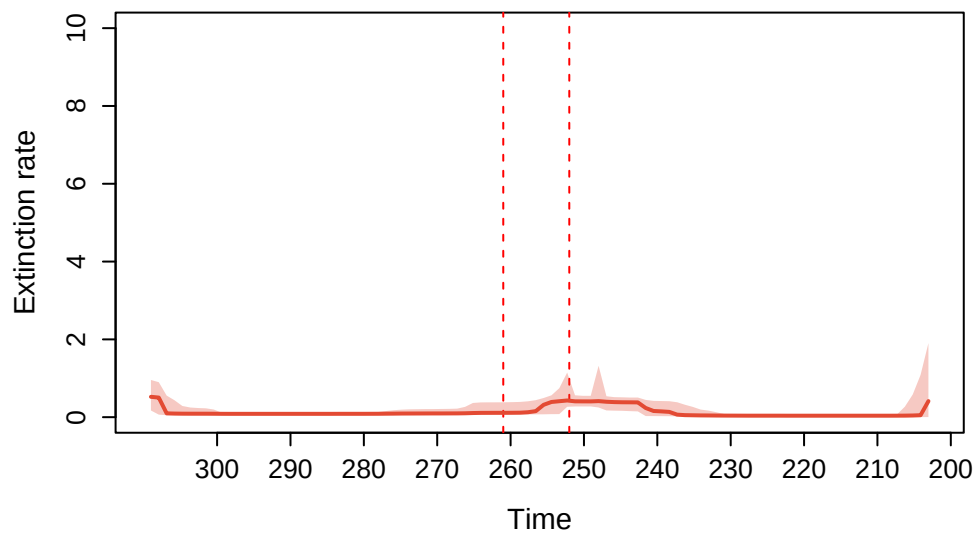
Extinction
