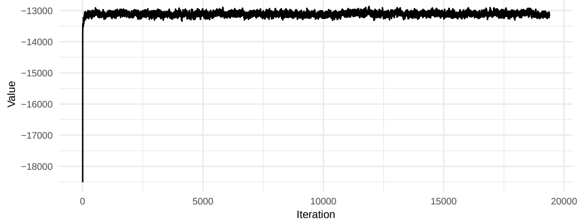
Prior Trace
