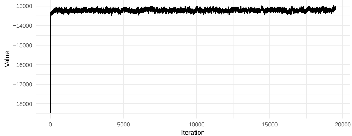
Prior Trace
