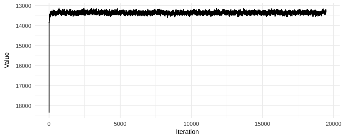
Prior Trace
