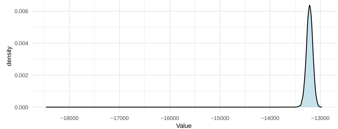
Prior Density
