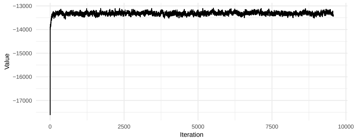
Prior Trace
